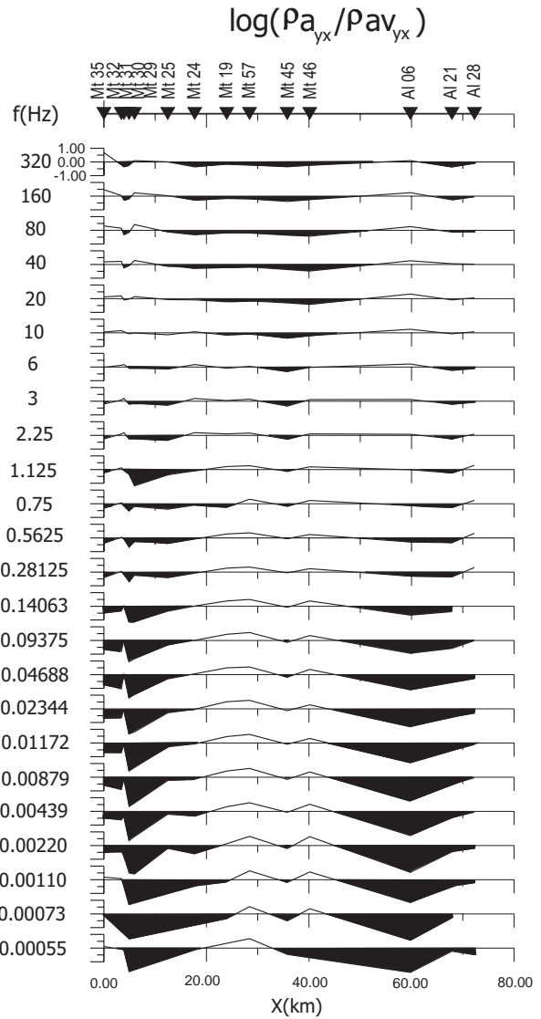
Figure 4. Profiles of logarithm of residual resistivity at 24 fixed frequencies at 14 stations along the E-W direction.
