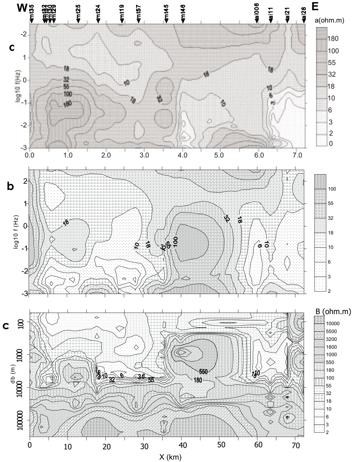
Figure 2. The MT apparent resistivity-frequency ( \rho_a , f ) pseudosections in (a) N-S, (b) E-W directions, and (c) Bostick resistivity-depth ( \rho_b , db ) transformation of the E-W apparent resistivity data along profile M1.
