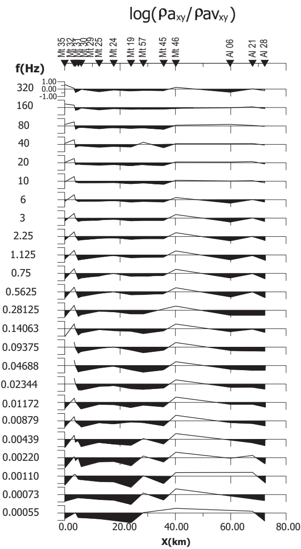
Figure 3. Profiles of logarithm of residual resistivity at 24 fixed frequencies at 14 stations along the N-S direction.
