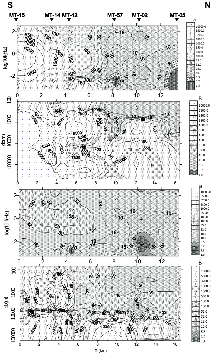
Figure 6. (a) MT apparent resistivity pseudosections in the E-W direction; (b) its Bostick depth transformation in the E-W direction; (c) The MT apparent resistivity pseudosections in the N-S direction; and (d) its Bostick depth transformation in the N-S direction along profile M2.
