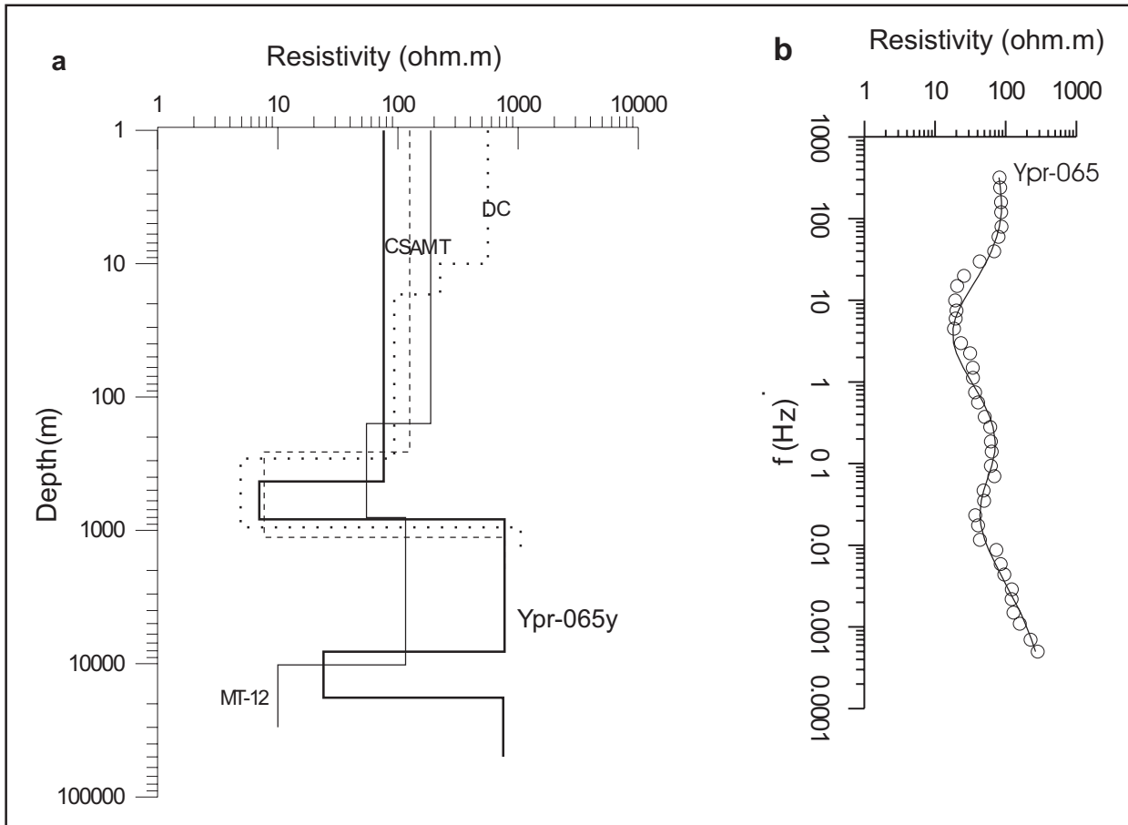
Figure 5. (a) 1D inversion results from co-located DC (Direct Current) resistivity, CSAMT (Controlled Sourced Audio Frequency Magnetotelluric), and MT (Magnetotelluric) soundings from sites MT-12 and ypr-65; and (b) The actual response of the Earth to the sounding at MT site ypr-65 (circles) and the best-fit model response (solid curve) to the field data.
