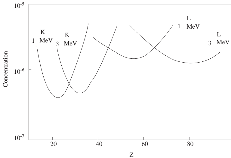
Figure 8. Minimum detectable concentration as a function of atomic number for protons of 1 and 3 MeV 10 .
