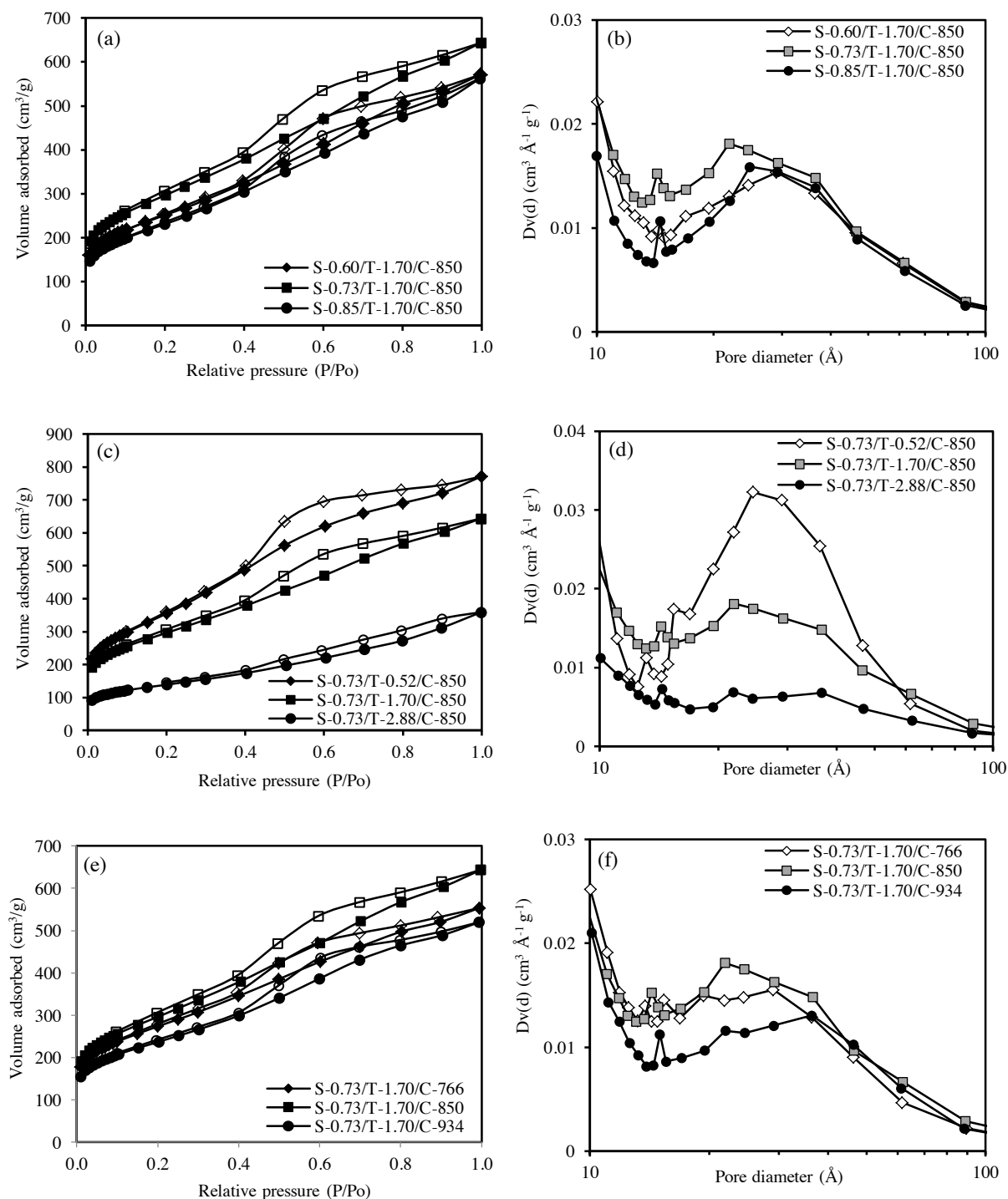
Figure 5. The adsorption-desorption isotherms (a, c, e) and pore size distributions (b, d, f) of porous carbons.
