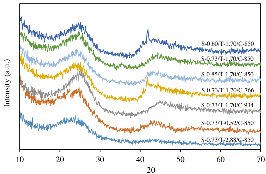
Figure 2. XRD patterns of porous carbons.
