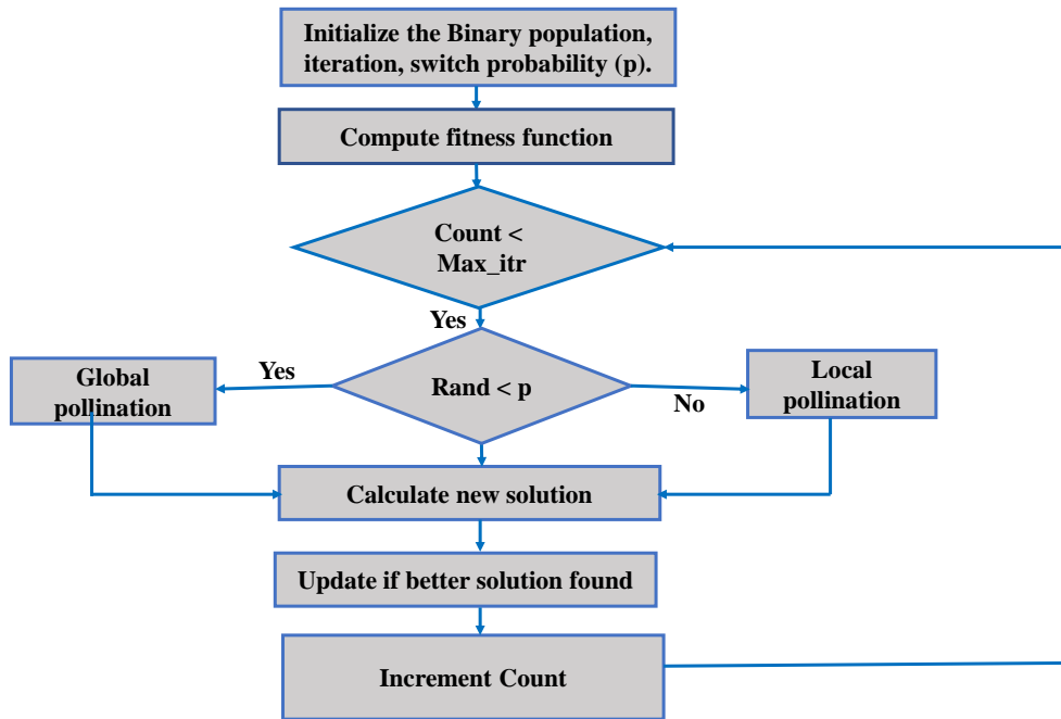
Figure 2. Framework of binary FPA.
