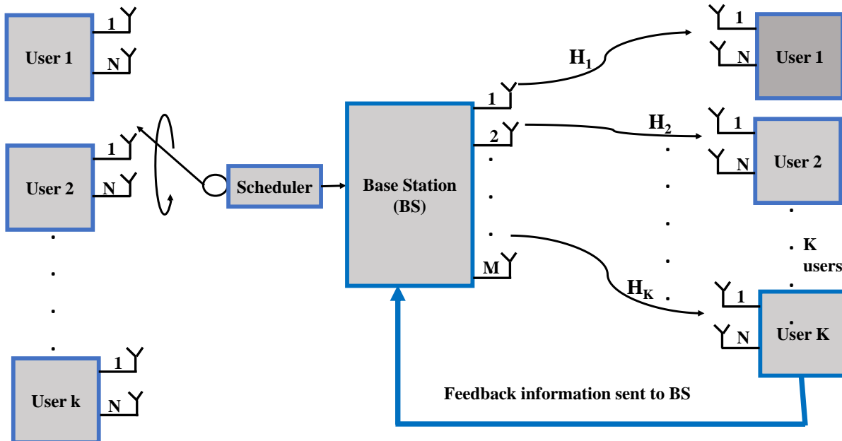
Figure 1. The MU MIMO system model for downlink transmission with M transmit antennas, K users each with N receive antennas.
