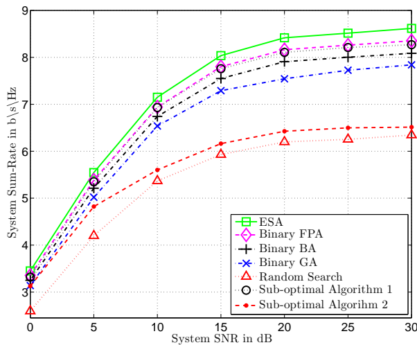
(a) K = 20, N = 4, M = 6, Pop\_size = 20, and Max\_itr = 30.
