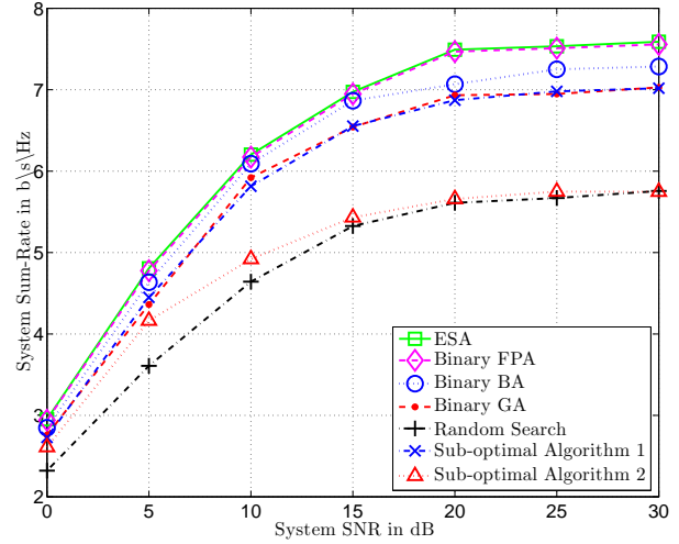
(b) K = 12 , N = 3 , M = 5 , Pop\_size = 12 , and Max\_itr = 30 .
