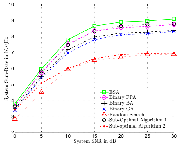
(b) K = 25, N = 5, M = 7, Pop\_size = 25, and Max\_itr = 30.
