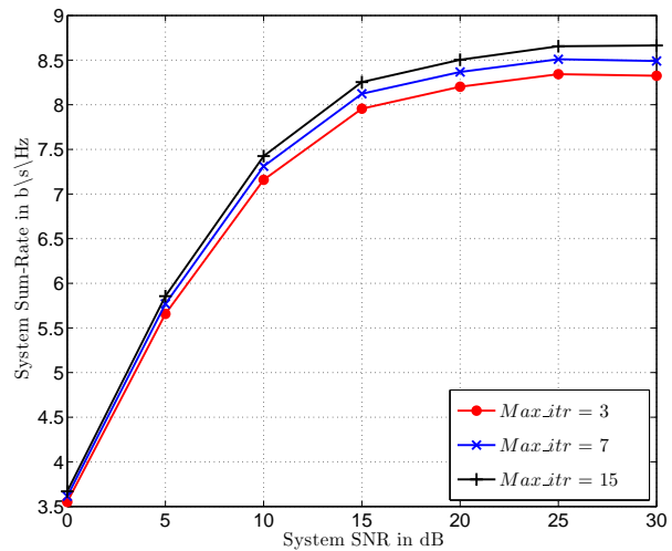
(b) K = 30 , N = 6 , M = 8 , Pop\_size = 5 , and Max\_itr = 3, 7, \text{ and } 15 .
