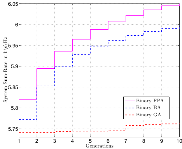
(a) K = 10, N = 3, M = 4, Pop\_size = 10, Max\_itr = 10, and SNR = 10 dB.
