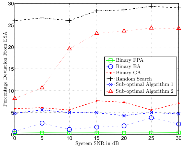
(a) K = 10 , N = 2 , M = 4 , Pop\_size = 10 , and Max\_itr = 30 .
