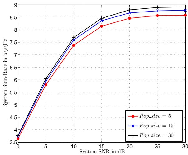
(a) K = 30 , N = 6 , M = 8 , Max\_itr = 10 , and Pop\_size = 5, 15, \text{ and } 30 .
