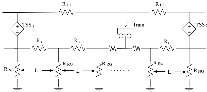
Figure 1. A simple model that can be used for computer simulations of stray currents.
