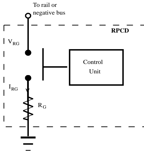
Figure 6. Schematic diagram of the RPCD.
