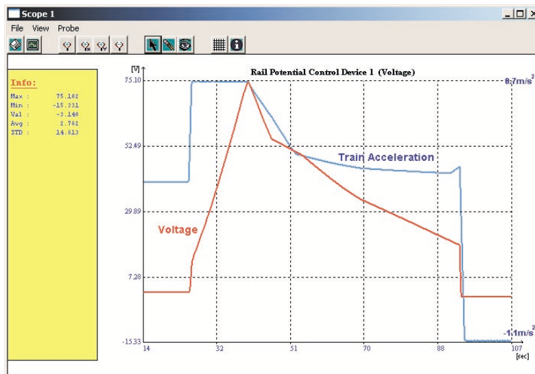
Figure 5. Change in train acceleration and rail voltage at the first passenger station with no RPCDs installed.
