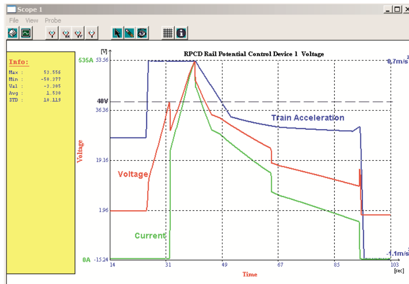
Figure 8. Change in voltage and current on RPCD1 during the acceleration period of the train for V_r = 40 V.
