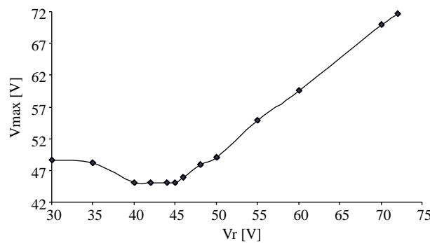
Figure 10. Maximum rail voltage vs. voltage threshold of RPCDs ( V_r ) for R_G = 0.08 \Omega .
