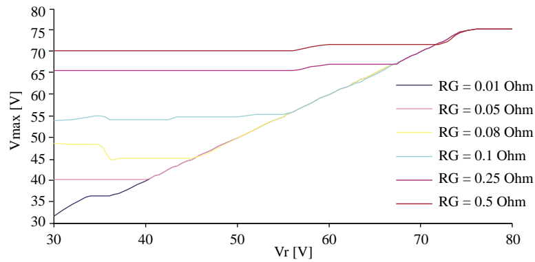
Figure 11. Maximum rail voltages for different settings of V_r and R_G for the simulation study case.
