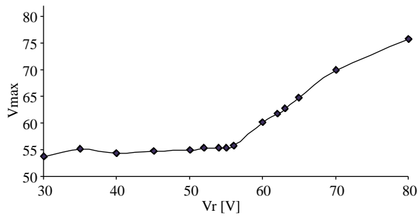
Figure 9. Maximum rail voltage vs. voltage threshold of RPCDs ( V_r ) for R_G = 0.1 \Omega for the simulation study case.
