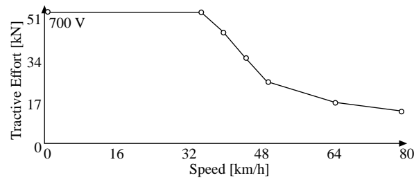
Figure 4. Tractive Effort (kN) – Speed (km/h) of the train set in the simulation case.
