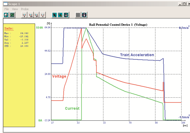
Figure 7. Change in voltage and current on RPCD1 during the acceleration period of the train.
