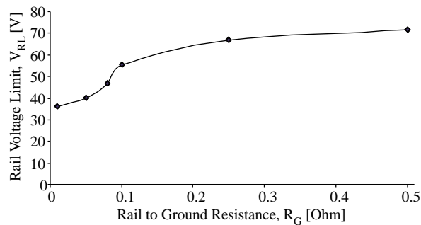
Figure 12. Rail voltage limit ( V_{RL} ) vs. rail to ground resistance ( R_G ) for the simulation study case.
