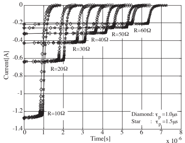
Figure 9. The reverse-recovery current transient curves of the p^+n diode for 1.0 \mu s and 1.5 \mu s ifetime after a forward current of 1.209 A.
