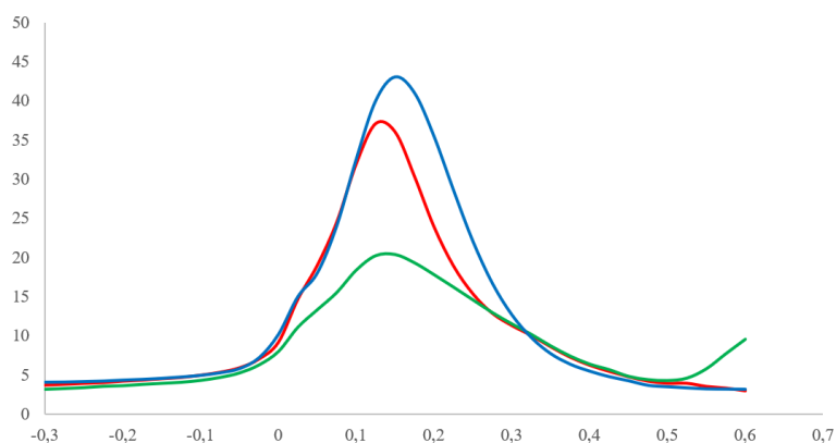
Potentials (V)
