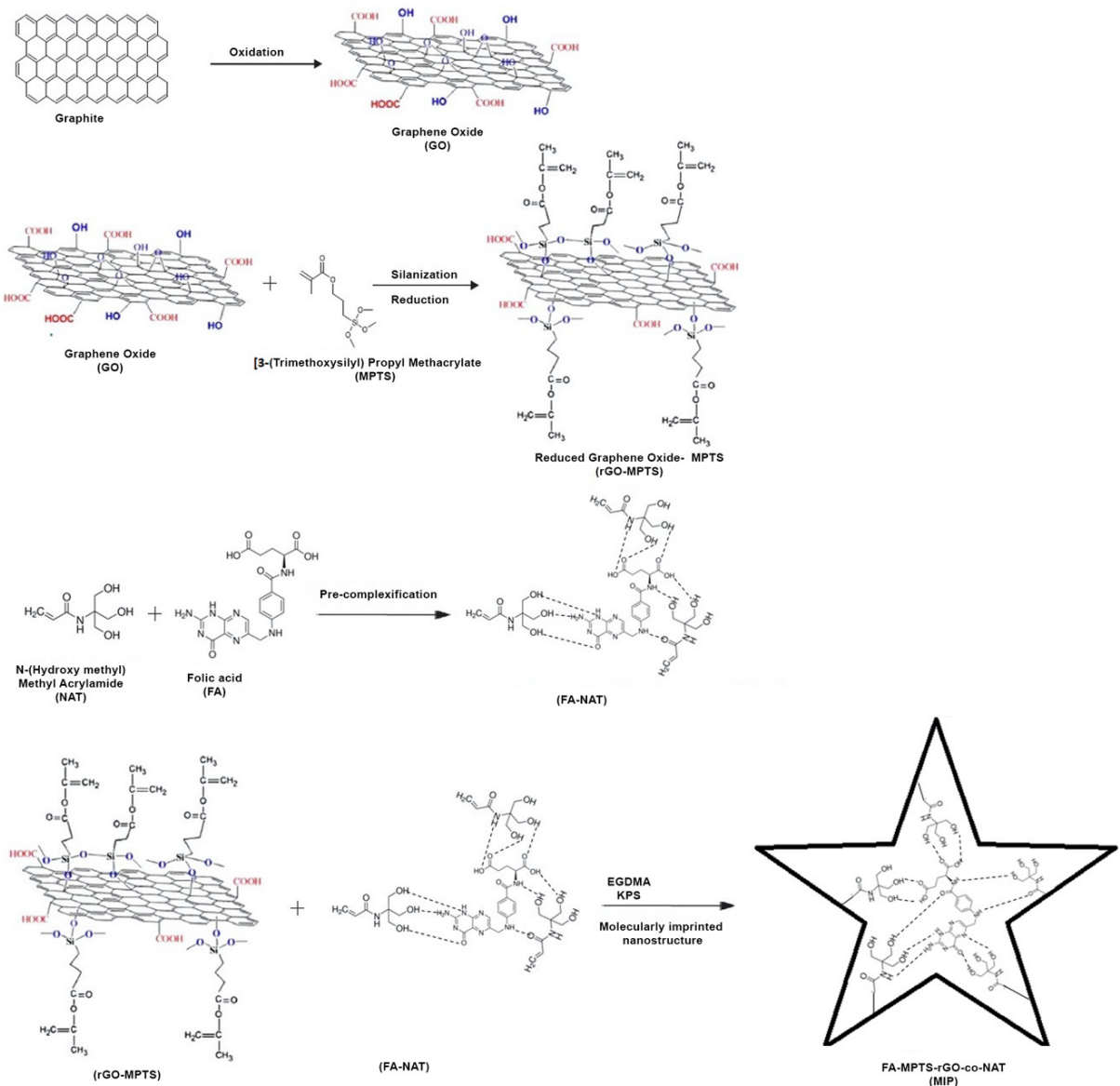
Figure 2. Synthesis steps and possible chemical interactions of FA-Imp-poly(MPTS-rGO-co-NAT).
