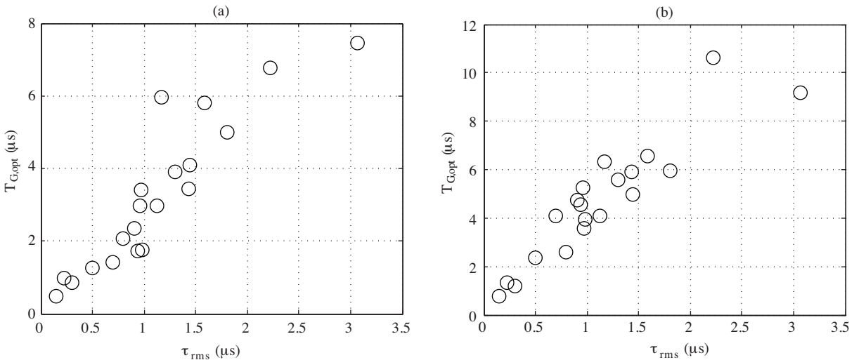
Figure 6. T_{G,opt} versus \tau_{rms} for 20 measured channel models for a) E_s/N_0 = 10 dB and b) E_s/N_0 = 20 dB.
