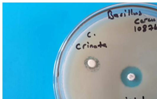
Figure 1. Antimicrobial test view of essential oil on B. cereus A:15 \mu L, B:30 \mu L, Tob: Tobramycin, Nys: Nystatin.
