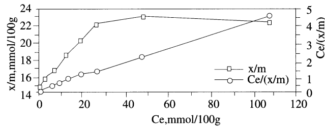
Figure 7. SP-MB adsorption isotherm and Langmuir line
