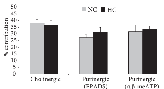
Figure 3. Contributions of cholinergic and purinergic (in the presence of PPADS ( 10^{-4} M) or \alpha,\beta -meATP ( 10^{-5} M)) components in contraction response of the rat detrusor smooth muscles to EFS in the control (NC; N = 6) and cholesterol (HC; N = 6) groups.
