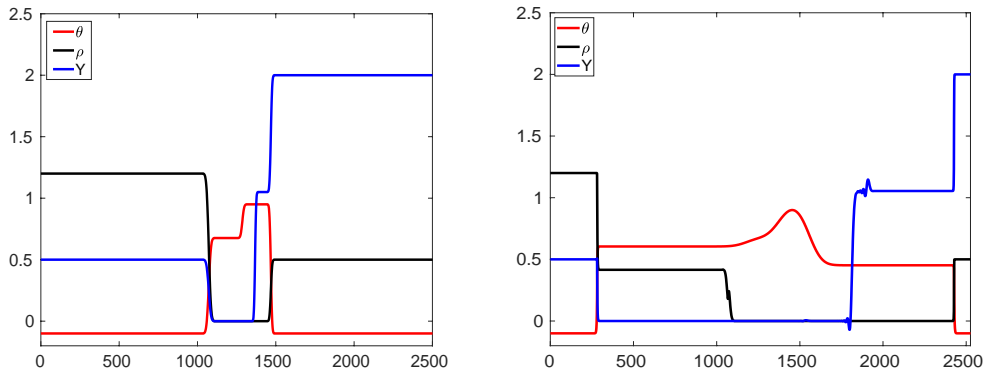
Figure 7. Result of numerical simulation yielding the wave sequence TC \xrightarrow{c_c} OC \xrightarrow{0} FC \cap OC \xrightarrow{a} FC \cap OC \xrightarrow{b} FC \xrightarrow{c_f} TC . Initial conditions (left) and simulation time 9000 (right).
