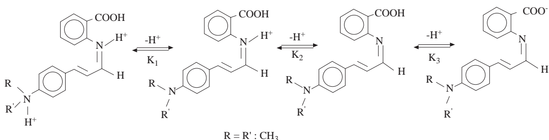
Figure 2. The ionization of the ligand (DACAB)
