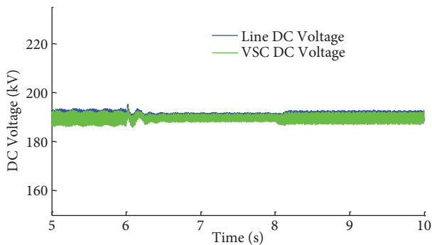
Figure 8. Voltages of the DC line and VSC DC bus.
