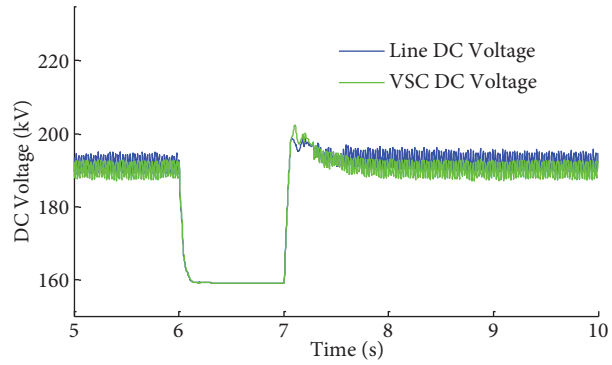
Figure 11. Voltages of the DC line and VSC DC bus when the DC line voltage drops by 20%.
