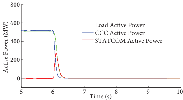
Figure 15. Active powers of the load, CCC, and STATCOM under DC voltage reduction when the capacitance of the STATCOM DC link is 0.2 mH.
