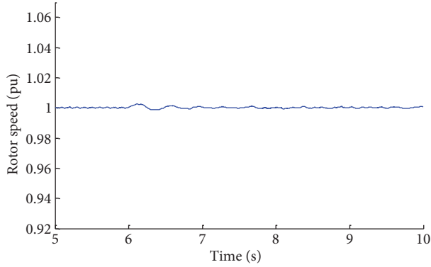
Figure 10. Rotor speed of the induction motor (pu).
