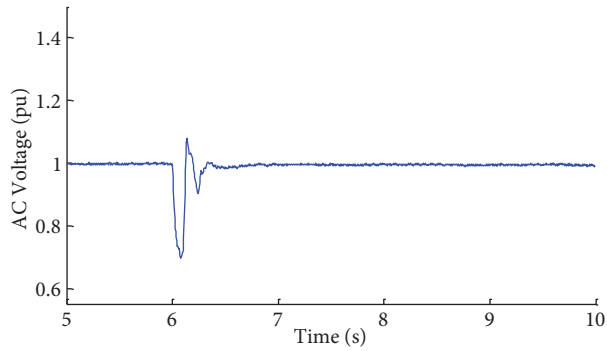
Figure 17. AC Voltage in per-unit under the short circuit fault.
