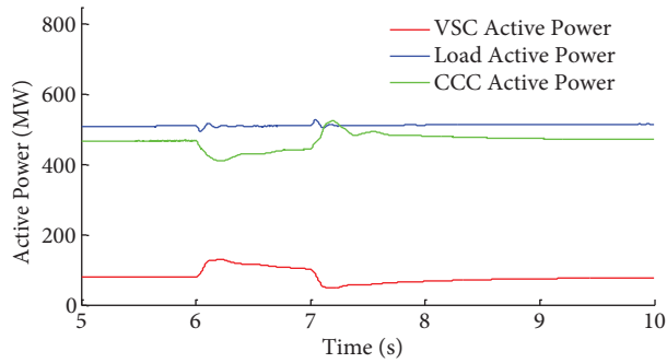
Figure 14. Active powers of the load, CCC, and VSC under DC voltage reduction when 2 separate DC lines are used.
