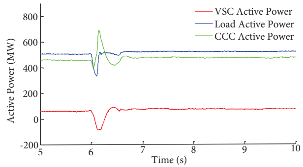
Figure 18. Active powers of the load, CCC, and VSC under the single-phase short-circuit fault when the network is infed by the proposed system (1 DC line is used for both converters).
