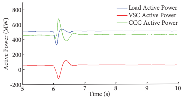
Figure 19. Active powers of the load, CCC, and VSC under the single-phase short-circuit fault when 2 separate DC lines are used for converters.
