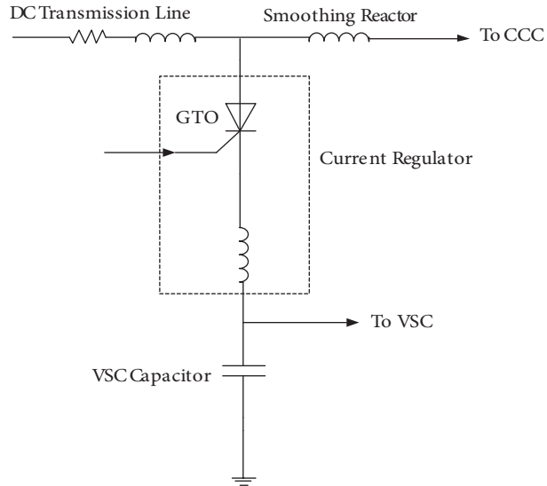
Figure 3. Current regulator.
