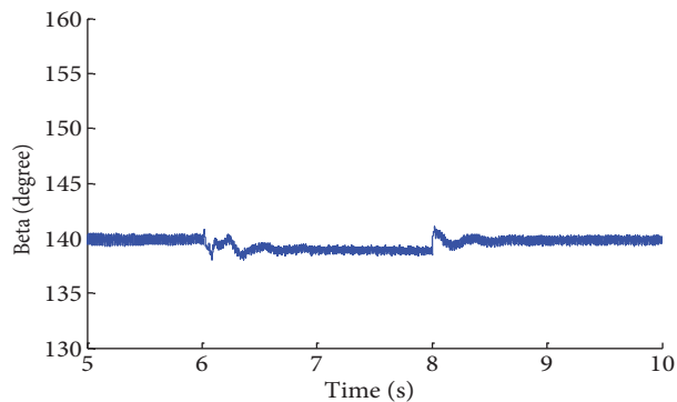
Figure 9. CCC firing angle.
