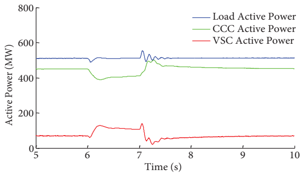
Figure 12. Active powers of the load, CCC, and VSC when the DC line voltage drops by 20%.
