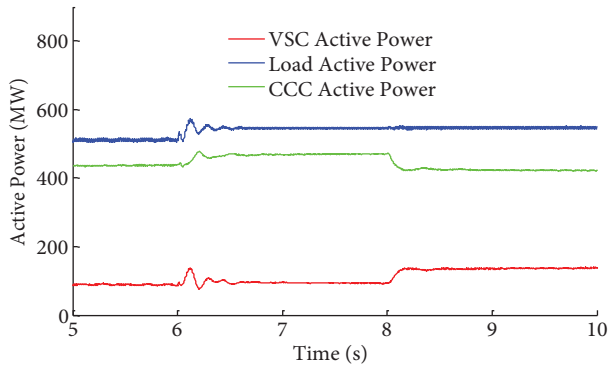
Figure 6. Active powers of load, CCC, and VSC.
