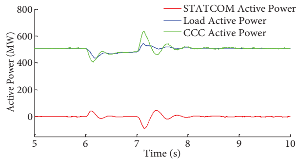
Figure 16. Active powers of the load, CCC, and STATCOM under DC voltage reduction when the capacitance of the STATCOM DC link is 2.0 mH.
