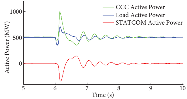
Figure 20. Active powers of the load, CCC, and STATCOM under the single-phase short-circuit fault.
