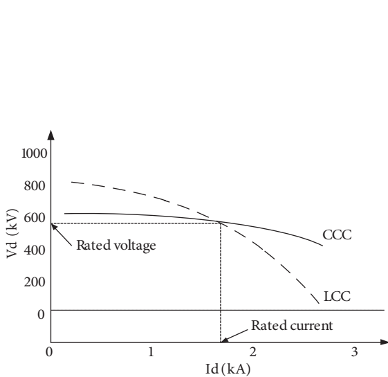
Figure 2. DC current-voltage characteristics of the CCC and LCC [19].
