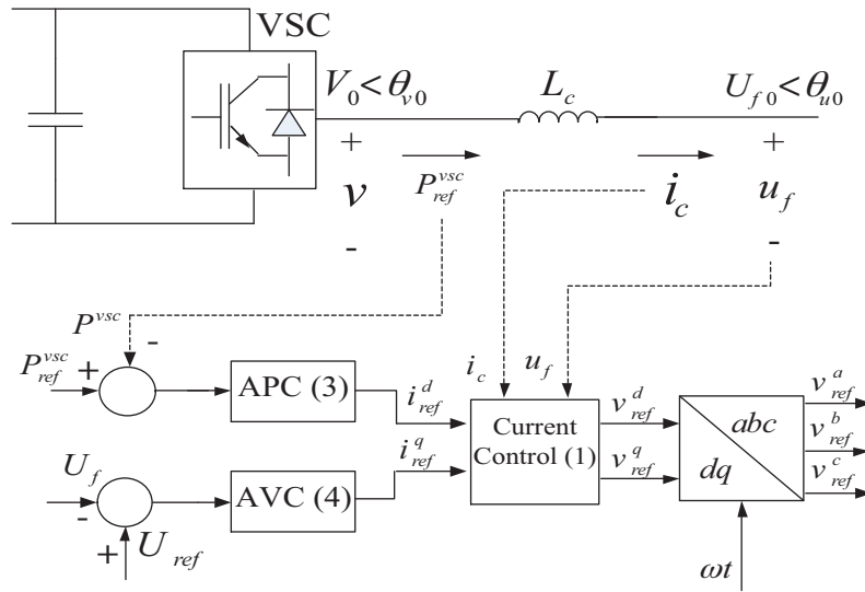
Figure 4. Main circuit and control block diagram of the VSC using current vector control.
