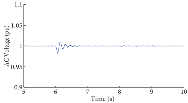
Figure 7. The network AC voltage.
