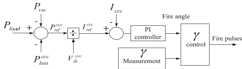
Figure 5. Control block-diagram of the CCC.
