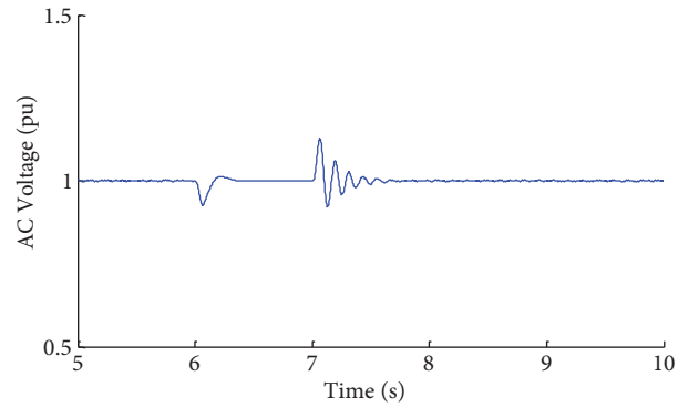
Figure 13. AC voltage of the network when the DC line voltage drops by 20%.
