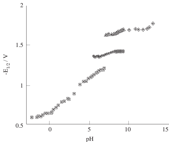
Figure 4. Dependence of half-wave potentials (SCE) on pH in buffered solutions of 2 \times 10^{-4} M maleic hydrazide for \square , wave I 1 ; \circ , wave I 2 ; \Delta wave I 3 ; \diamond , wave I 4 . Reprinted from Journal of Electroanalytical Chemistry 420, 79-87 (1997).
