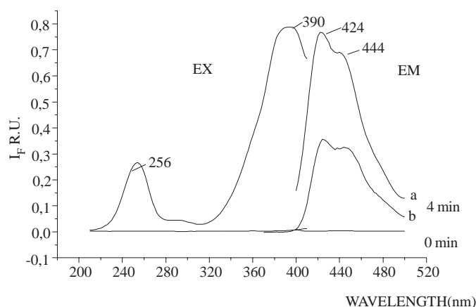
Figure 1. PIF excitation (EX) and emission (EM) spectra of flufenamic acid ( 10^{-5} M) in a 0.1M \text{HClO}_4 aqueous solution (pH = 1.0 ; t_{irr} = 4 min). Emission spectra were recorded at \lambda_{ex} = 390 nm (curve a) and 256 nm (curve b), respectively. Corresponding spectra are also given below for t_{irr} = 0 min.
