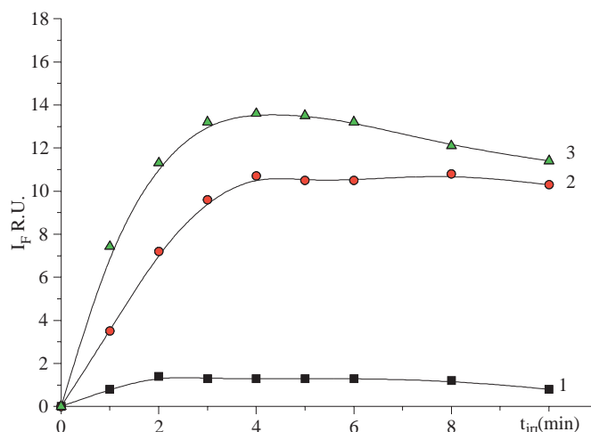
Figure 2. Influence of the UV irradiation time on the PIF intensity of flufenamic acid at concentrations of 0.3 ng/mL (curve 1) 3.0 ng/mL (curve 2) and 41 ng/mL (curve 3) in acidic (pH = 1) aqueous solutions. The curve corresponding to 41 ng/mL was obtained with a sensitivity scale divided by 10.
