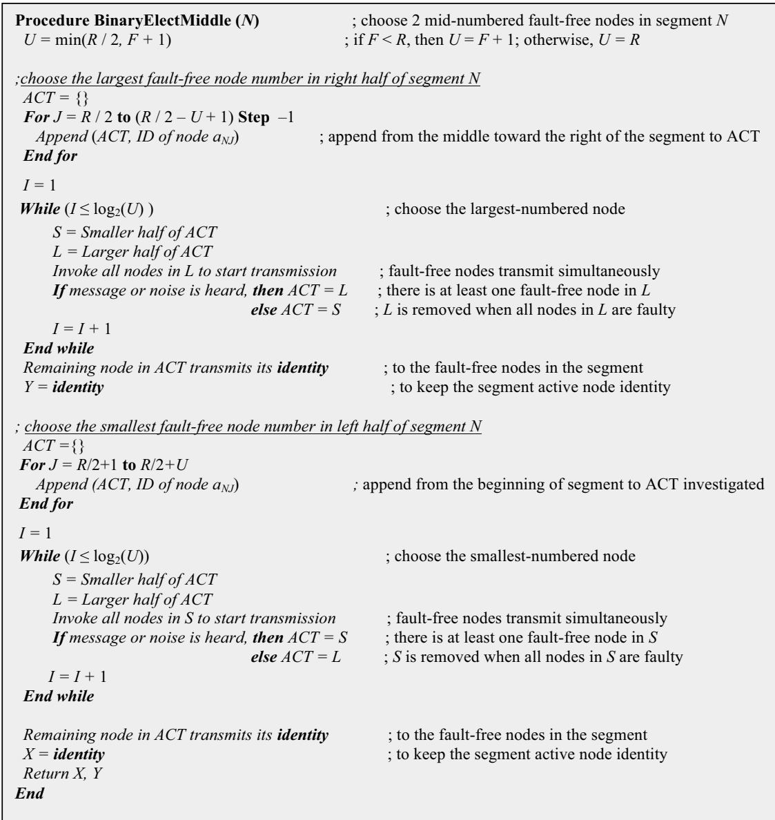
Figure 9. The BinaryElectMiddle algorithm.
