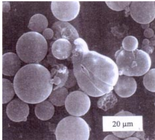
Figure 2. The photograph, taken by a scanning electron microscope, of the fine powders which were obtained by the calcination of the alumina precursor for 2 hours at 1000^\circ\text{C} .
