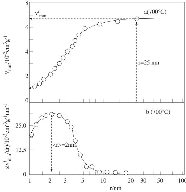
Figure 7. a) v_{mm}^l - r and b) dv_{mm}^l/dr - r pore size distribution curves which were determined from the desorption data.
