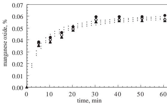
Figure 7a. The change in manganese oxide solubility with USP and sonication time (for samples grain size 1 and mass 0.0500 g) ●; maximum USP, ○; medium USP, ▲; minimum USP
