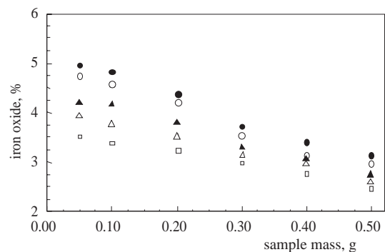
Figure 10b. The change in iron oxide solubility with sample grain size and sample masses (maximum USP and mean values from 30 to 60 min) ●; grain size 1., ○; grain size 2., ▲; grain size 3., △; grain size 4., ■; grain size 5.
