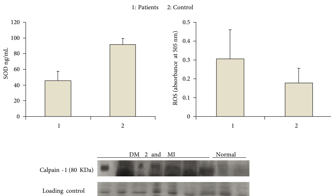
Figure 1. SOD, ROS, and calpain expression in diabetic and myocardial infarction patients. a) SOD activity in diabetic and MI patients (1) and normal individuals (2): reaction mixture containing L-methionine, NBT, and Triton was illuminated with a fluorescent lamp. After addition of riboflavin, SOD activity was analyzed in serum samples at 560 nm. b) ROS concentrations in diabetic and MI patients (1) and normal individuals (2). The DEPPD method was employed for detecting ROS at 505 nm, relating high absorbance rate with increased ROS concentrations. c) Blot analysis of calpain-1 in serum of diabetic MI patients. The 6 left-side lanes represent calpain expression in diseased samples and the extreme 2 right lanes represent normal healthy controls.
