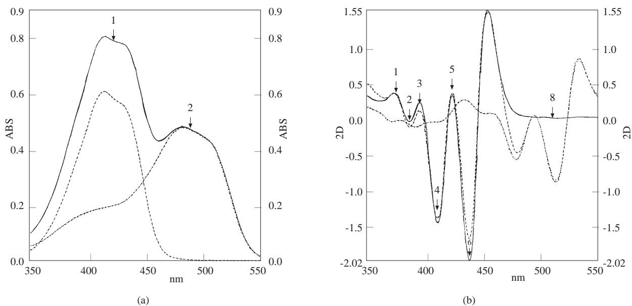
Figure 1. a) Absorption spectra for solutions of 10 \mu\text{g ml}^{-1} of QY (---), SY (-.-.-) and their mixture (—), recorded against a blank of acetate buffer (pH = 4.5)
