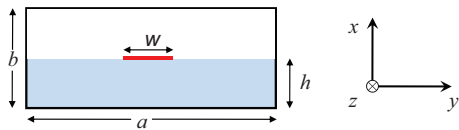
Figure 9. Microstrip line.
