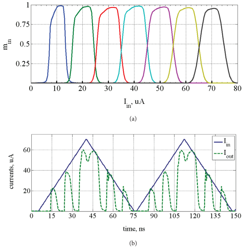
Figure 2. (a) Membership function DC characteristics of the proposed MFC for seven fuzzy sets; (b) transient simulation results of the designed classifier with proposed MFC for k = 2, 4, and 6 .
