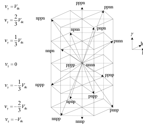
Figure 3. Switching vectors of a four-leg inverter.
