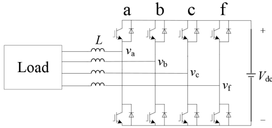
Figure 2. Four-leg inverter topology.
