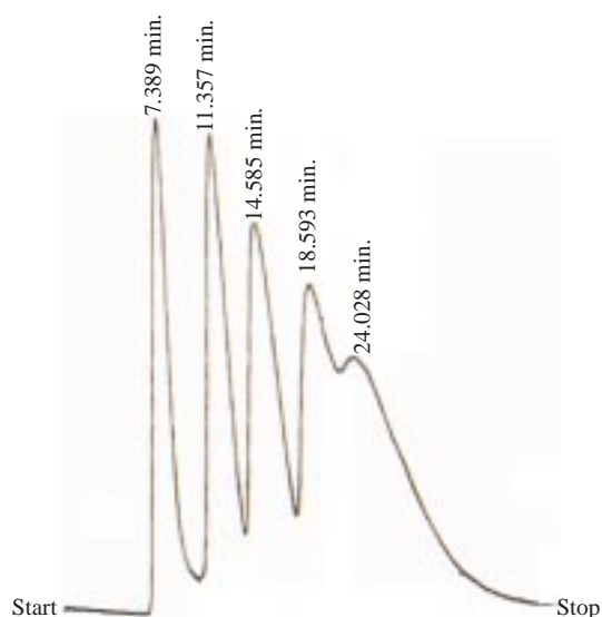
Figure 1. Gas Chromatogram of phenol isomers mixture on 20% benzylidene-p-aminobenzoic acid Conditions: Oven Temp. = 190 °C, Flow rate = 40 mL/min, Det. and Inj. = 240 °C. Sample size 1 \mu L. Peaks: 1 = Ethanol (solvent), 2 = 2,6-dimethyl phenol, 3 = 2,5-dimethyl phenol, 4 = 3,4-dimethyl phenol, 5 = 3,5-dimethyl phenol.
