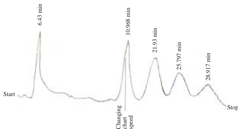
Figure 2. Gas Chromatogram of phenol isomers mixture on 20% p-methyl benzylidene-p-aminobenzoic acid Conditions: Oven Temp. = 256 °C, Flow rate = 30 mL/min, Det. and Inj. = 270 °C. Sample size 1 \mu L. Peaks: 1 = Ethanol (solvent), 2 = 2,6-dimethyl phenol, 3 = 2,5-dimethyl phenol, 4 = 3,4-dimethyl phenol, 5 = 3,5-dimethyl phenol.
