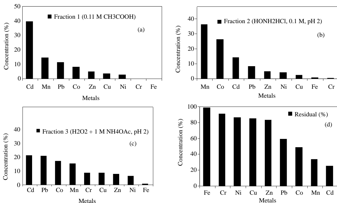
Figure 2. Extractability order of the metals in each extraction stage of the BCR sequential extraction procedure and residual phase for 21 soil samples.
