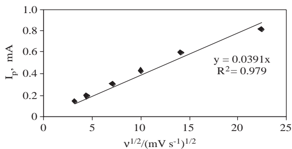
Figure 3. The change of peak current with the scan rate on glassy carbon electrode.
