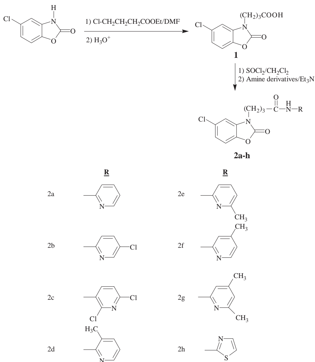
Scheme 1. Synthetic route for the synthesis of the title amide derivatives.
