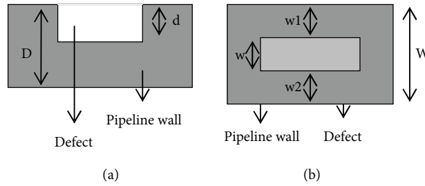
Figure 6. (a) Side view of defect in pipeline, (b) top view of defect in pipeline.
