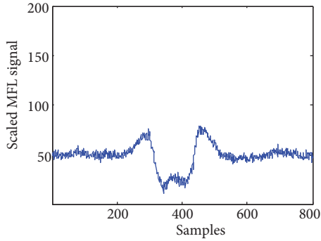
Figure 4. MFL signal for the placement of a clamp in the pipeline.
