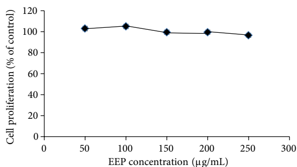
Figure 1. Effect of EEP on fibroblast cell viability shown by the MTT reduction test. Fibroblast cells were incubated for 24 h with increasing concentrations of EEP. Control cells were incubated in the presence of 1% ethanol. Values represent mean \pm SD based on results obtained in at least 3 independent experiments.
