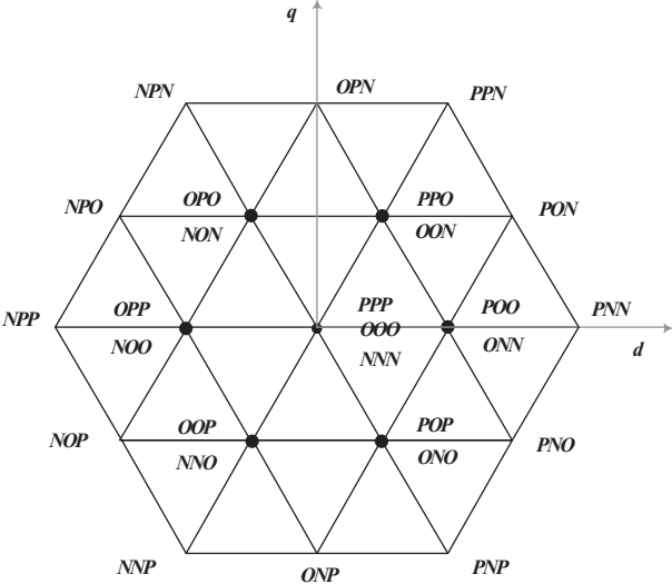
Figure 15. Space vector diagram of 3-level converter.
