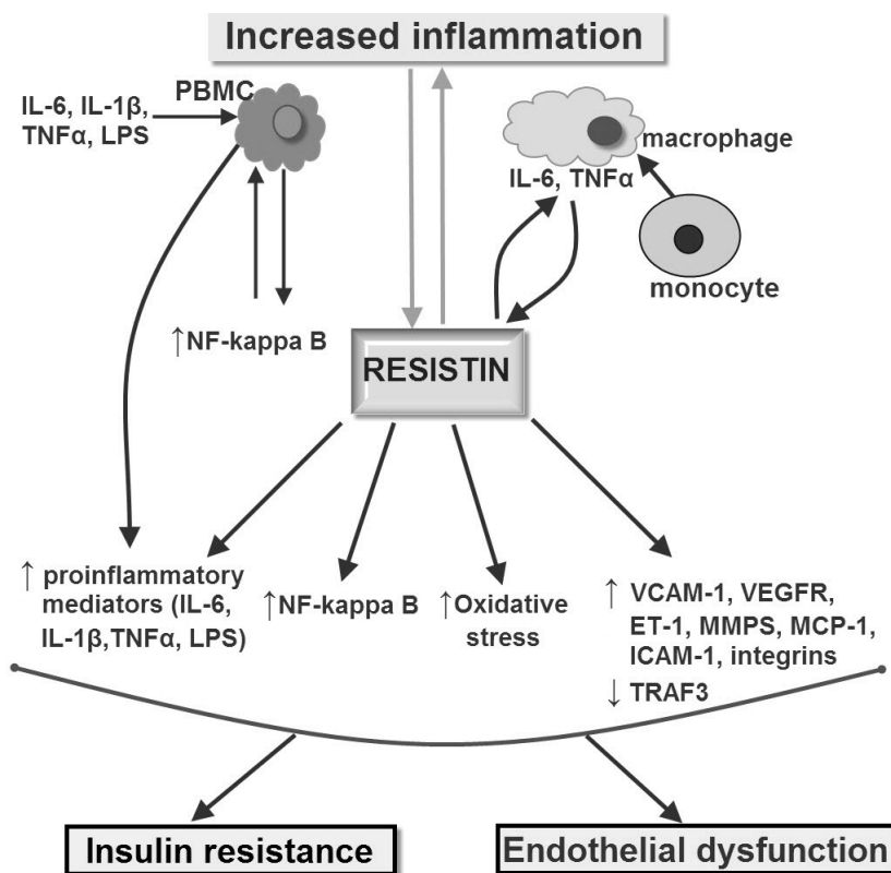
Figure 4. Schematic representation of resistin as a potential regulatory molecule of inflammatory processes. Based on the cellular milieu, release of resistin acts as a signaling pathway in immune cells. Moreover, resistin has many unique features of the proinflammatory cytokines, which activates the transcription factor NF- \kappa B. The maturation/differentiation stage of monocytes/macrophages also upregulates resistin expression that increases after TNF- \alpha , IL-6, IL-1 \beta , and LPS stimulation. VCAM-1, vascular cell adhesion molecule; TRAF3, TNF receptor-associated factor-3; PBMCs, peripheral blood mononuclear cells; ICAM-1, intercellular adhesion molecule 1; ET-1, endothelium-derived vasoactive factor; TNE, tumor necrosis factor; IL, interleukin; VEGFR, vascular endothelial growth factor receptor; MCP-1, monocyte chemoattractant protein; MMPs, matrix metalloproteinases; LPS, lipopolysaccharide; NF- \kappa B, nuclear factor kappa B.
