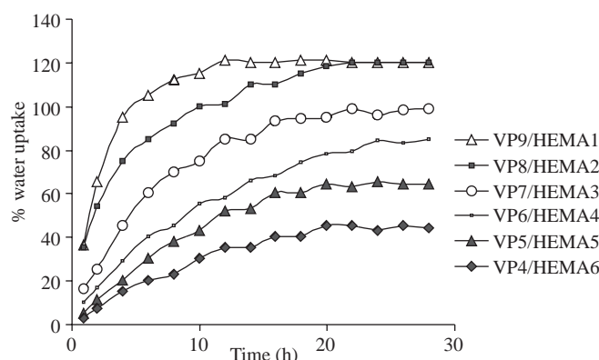
Figure 1. Variation of percentage water uptake with time (h) for various compositions of VP/HEMA copolymer.
