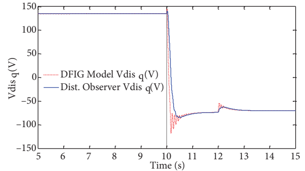
Figure 10. Estimated and modeled disturbance terms ( v_{disq} ).
