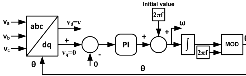
Figure 2. PLL algorithm.
