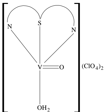
Figure 2. Probable structure of [VO(L_2)](ClO_4)_2 complexes; L = 4'-NO_2BAAPTS or FFAAPTS ).
