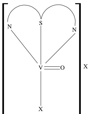
Figure 1. Probable structure of [VO(L)X]X complexes; ( X = Cl, Br, NO_3 or NCS and L = 4'-NO_2BAAPTS or FFAAPTS ).
