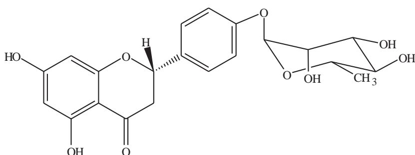
Naringenin-4' O- \alpha -L-rhamnopyranoside (2)
