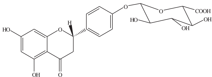
Naringenin 4'-O- \beta -D-glucuronopyranoside (1)
