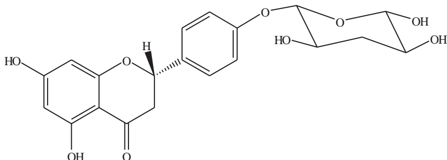
Naringenin-4'-O- \beta -D-xylopyranoside (3)
