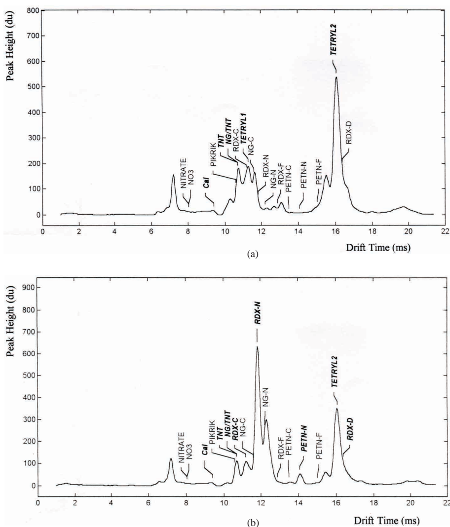
Figure 5. The plasmagrams of the standard mixture (a) and the handswab sample (b).
