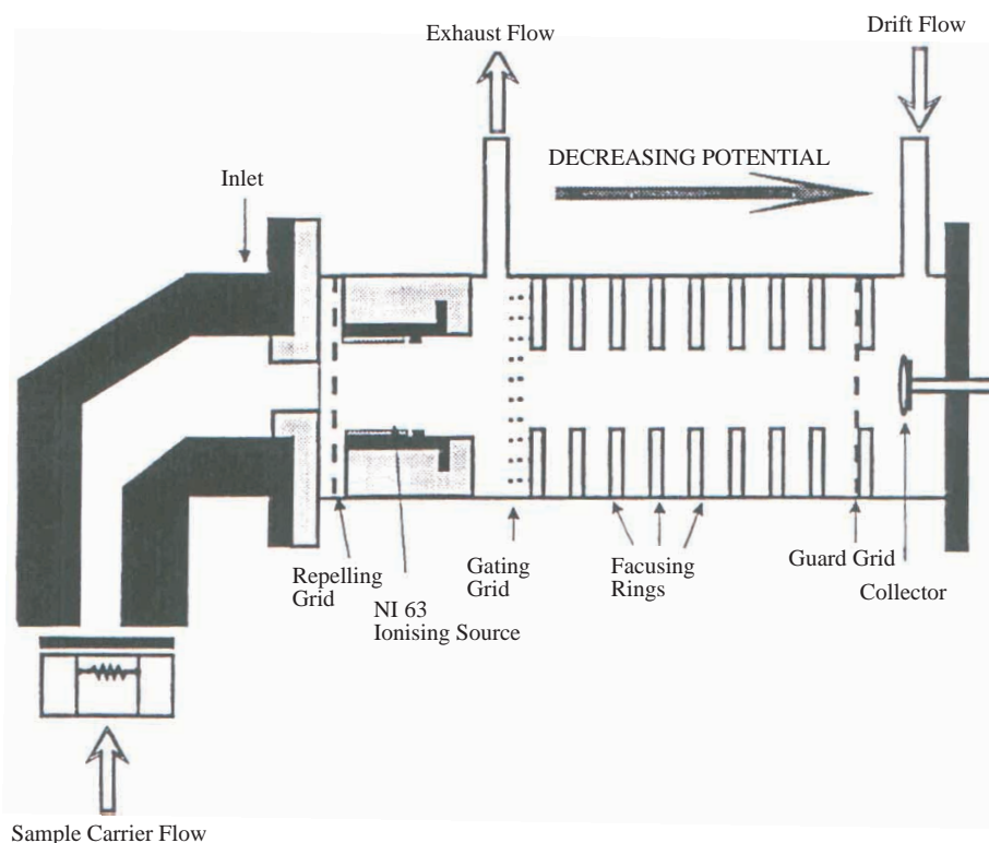
Figure 1. Schematic representation of an IMS detector cell.
