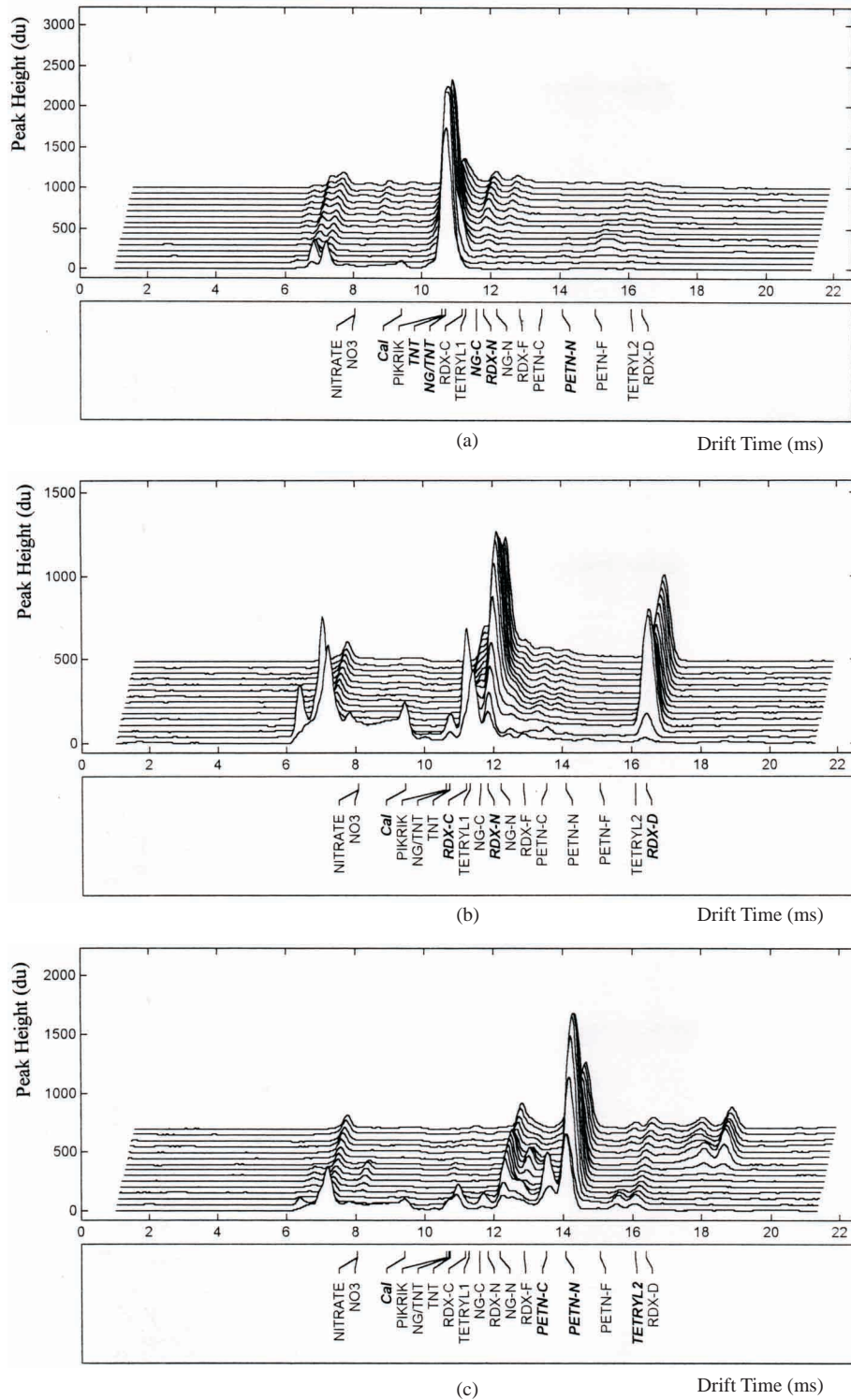
Figure 4. The plasmagrams of the TNT standard (a), RDX standard (b), PETN standard (c), TETRYL standard (d) and the acetone extract (e).
