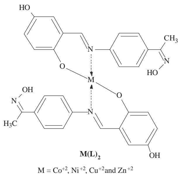
Figure. Suggested structural formula of the tetrahedral complexes of the ligand.
