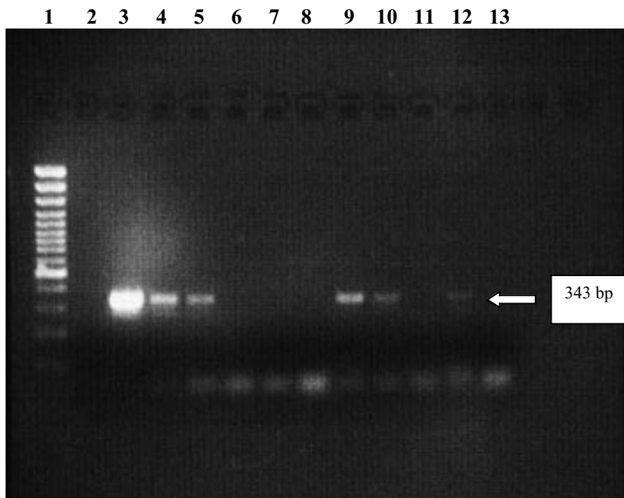
Figure 1. PCR assay for Listeria monocytogenes (specific amplification of the 343 bp fragment from the total DNA of Listeria monocytogenes ). Lane 1: 1-kb plus DNA ladder (MBI Fermentas); Lane 2: no template (negative control); Lane 3: L. monocytogenes NCTC 11994 (serotype 4b) (positive control); Lanes 4 to 6 and 9 to 13: DNA from H. pomatia ; Lane 7: Listeria innocua ; Lane 8: Escherichia coli ATCC 25922.
