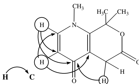
Figure. The significant long range correlation detected in the HMBC spectrum of compound 1 .
