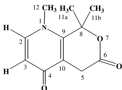
1,8,8-Trimethyl-5,8-dihydro-1H-pyrano[3,4-b]pyridine-4,6-dione
