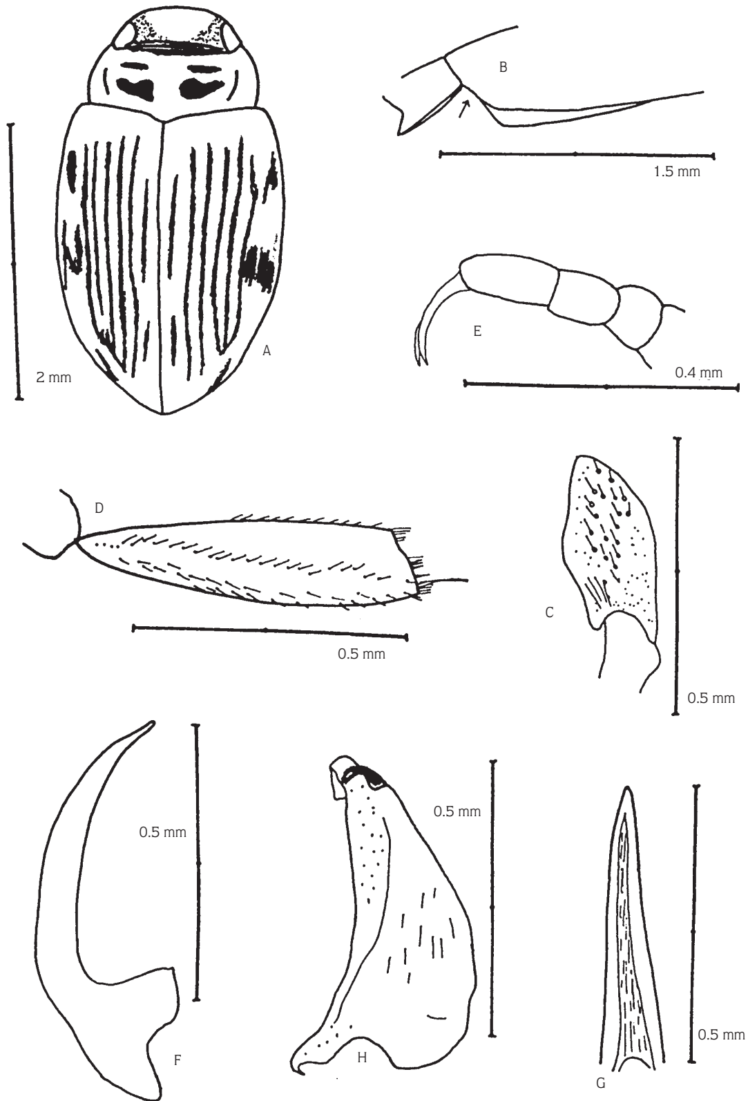
Figure 1. Oreodytes septentrionalis : Male: A) Habitus, B) Base of pronotum and elytron, lateral view, C) Metatrochanter, ventral view, D) Metatibia, ventral view, E) Protarsal claws, F) Aedeagus, lateral view, G) Aedeagus, dorsal view, H) Paramere.
