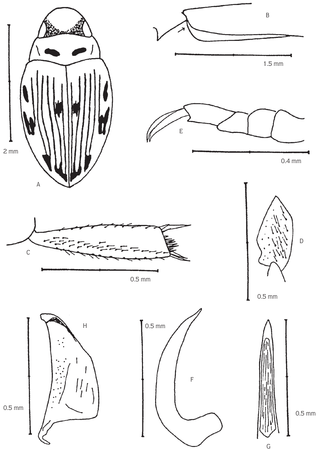
Figure 2. Oreodytes davisii : Male; A) Habitus, B) Base of pronotum and elytron, lateral view, C) Metatibia, ventral view, D) Metatrochanter, ventral view, E) Protarsal claws, F) Aedeagus, lateral view, G) Aedeagus, dorsal, H) Paramere.
