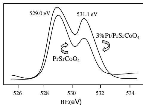
Figure 8. XPS patterns of O 1s of the PrSrCoO 4 and 3% Pt/PrSrCoO 4 catalysts.
