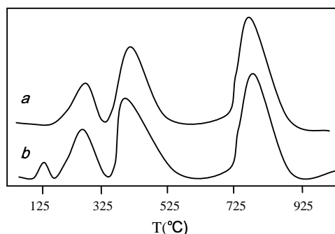
Figure 6. TPR patterns of the PrSrCoO 4 and 3% Pt/PrSrCoO 4 catalysts a: PrSrCoO 4 ; b: 3% Pt/PrSrCoO 4 .
