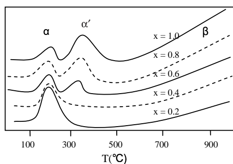
Figure 2. TPD patterns of the \text{Pr}_{2-x}\text{Sr}_x\text{CoO}_{4\pm\lambda} catalysts.
