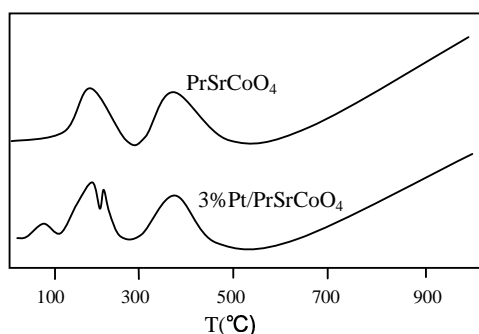
Figure 5. TPD patterns of the PrSrCoO 4 and 3% Pt/PrSrCoO 4 catalysts.
