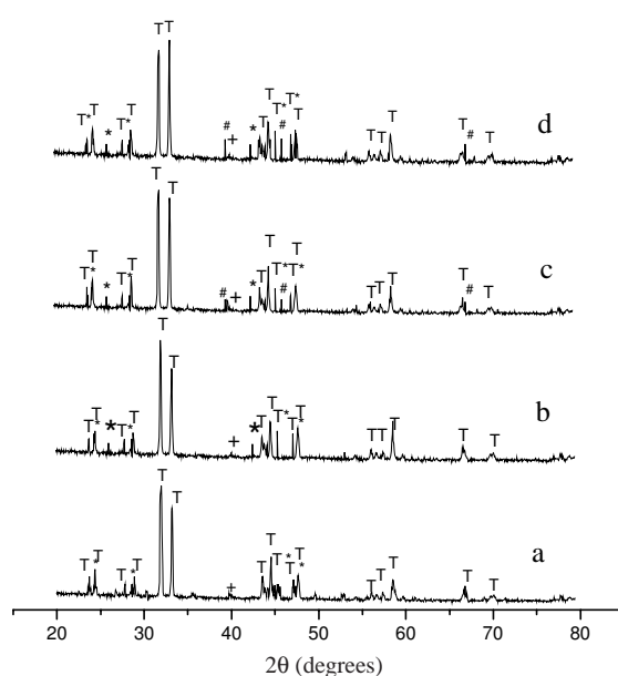
Figure 4. XRD patterns of the catalysts T: T phase, T*: T* phase, +:SrCO 3 , *:PtCl 4 , #: Pt. a: PrSrCoO 4 ; b: 1% Pt/PrSrCoO 4 ; c: 3% Pt/PrSrCoO 4 ; d: 5% Pt/PrSrCoO 4 .
