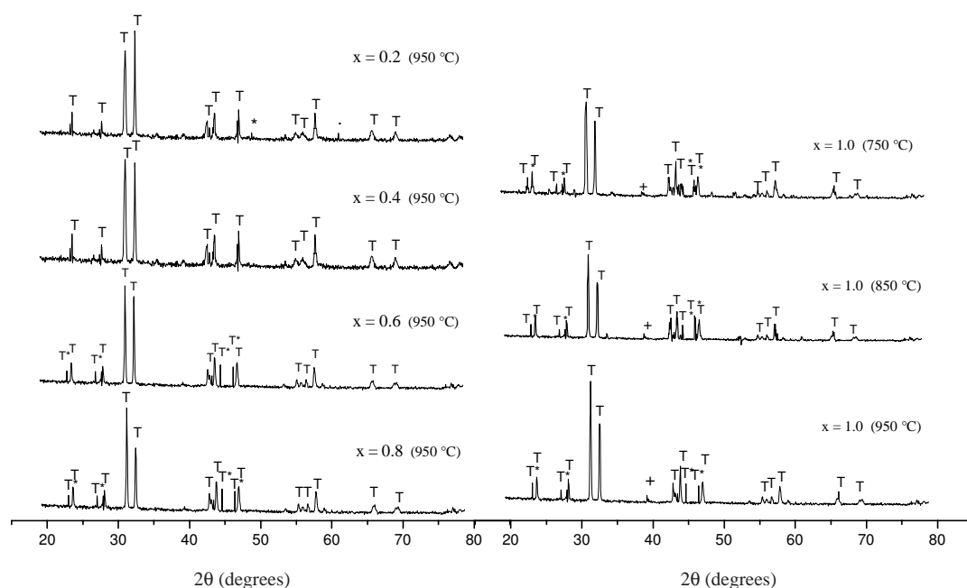
Figure 1. XRD patterns of the Pr 2-x Sr x CoO 4±λ catalysts T: T phase, T*: T* phase, +: SrCO 3 , *: Pr 2 O 3 , ·: CoO.
