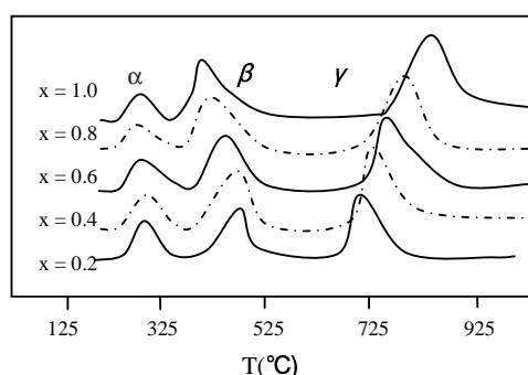
Figure 3. TPR patterns of the \text{Pr}_{2-x}\text{Sr}_x\text{CoO}_{4\pm\lambda} catalysts.
