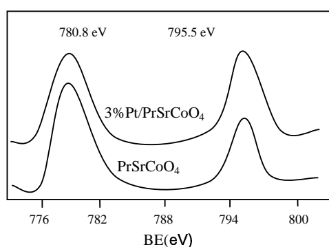
Figure 7. XPS patterns of Co 2p of the PrSrCoO 4 and 3% Pt/PrSrCoO 4 catalysts.
