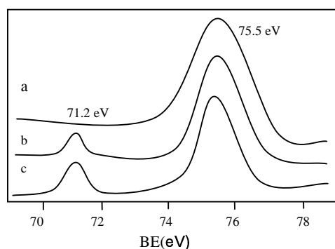
Figure 9. XPS patterns of Pt 4f of the Pt/PrSrCoO 4 catalysts a: 1% Pt/PrSrCoO 4 ; b: 3% Pt/PrSrCoO 4 ; c: 5% Pt/PrSrCoO 4 .
