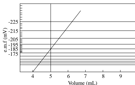
Figure 4. Multi-standard addition method for the determination of 0.01 M atenolol sample using Gran's plot paper with membrane IV.
