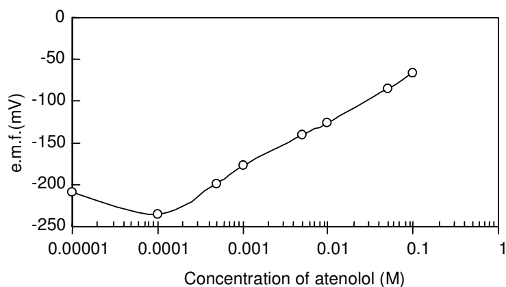
Figure 2. Calibration curve of atenolol selective electrode based on (A-TP) ionophore and DBPH plasticizer.
