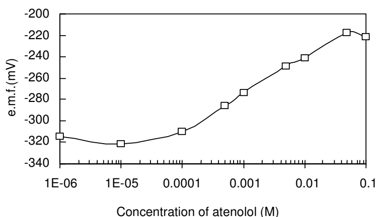
Figure 1. Calibration curve of atenolol selective electrode based on (A-TP) ionophore and DBP plasticizer.
