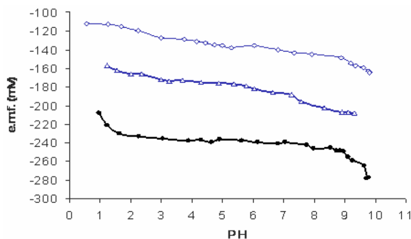
Figure 3. Effect of pH on response of the electrode IV at different atenolol concentrations. \circ - 10^{-2} M, \Delta - 10^{-3} M, \bullet - 10^{-4} M.
