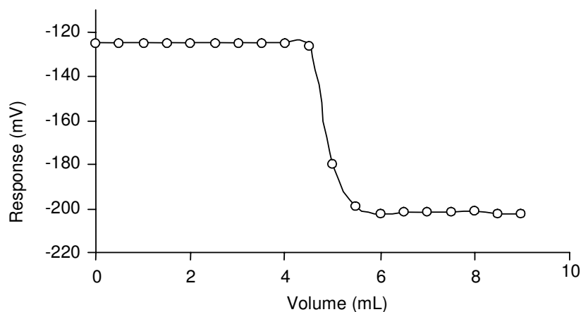
Figure 5. Titration curve for sample solution containing 5 mL of 0.01M atenolol with 0.01 M PT standard solution as titrant.
