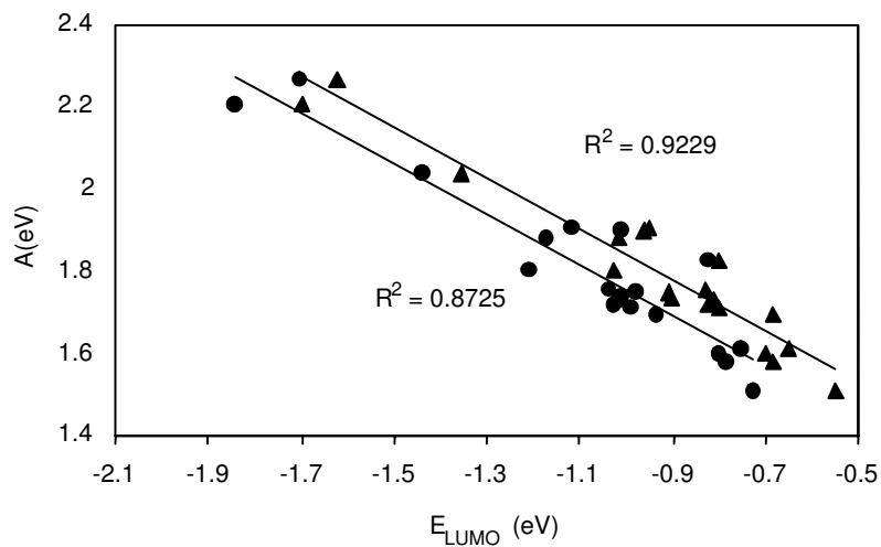
Figure 5. Plot of E_{LUMO} (calculated by PM3 \blacktriangle and AM1 \bullet methods) vs. electron affinity A .
