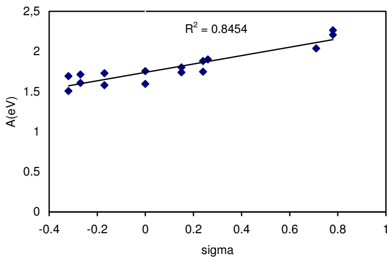
Figure 4. Plot of Hammett substituent constant ( \sigma ) vs. electron affinity ( A ).
