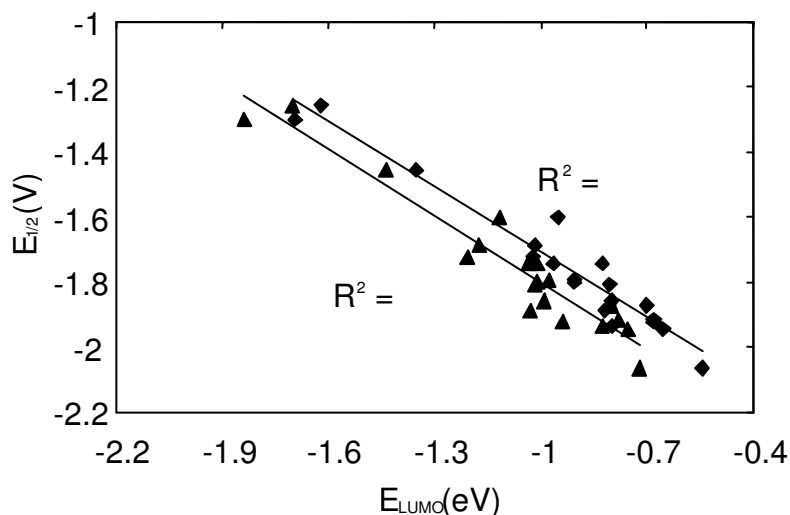
Figure 1. Plot of E_{LUMO} (calculated by AM1 ■ and PM3 ▲ methods) vs. E_{1/2} measured at scan rate 50 \text{ mVs}^{-1} .
