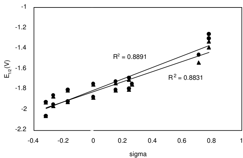
Figure 3. Plot of \sigma vs. E_{1/2} measured at scan rate 50 \bullet and 100 \blacktriangle mVs -1 .
