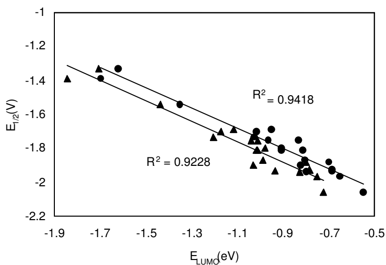
Figure 2. Plot of E_{LUMO} (calculated by AM1 ● and PM3 ▲ methods) vs. E_{1/2} measured at scan rate 100 \text{ mVs}^{-1} .
