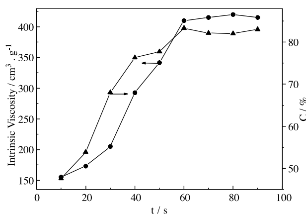
Figure 4. The effects of discharge time on intrinsic viscosity of Poly(MTAC) and conversion. Post-polymerization time 5 h, post-polymerization temperature 50 \pm 0.5^\circ , discharge power 60 W, MTAC mass fraction 0.25.
