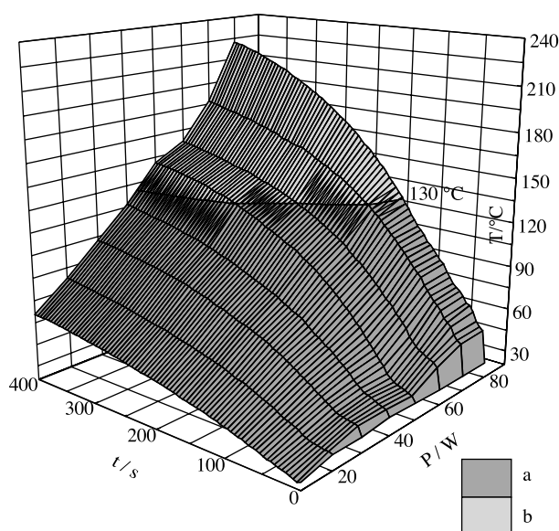
Figure 3. The effects of discharge time and discharge power on temperature in 133 Pa a: distribution of linear Poly(MTAC); b: distribution of cross-linked Poly(MTAC).
