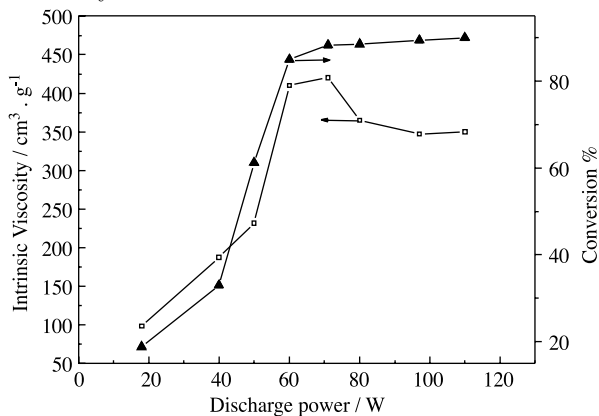
Figure 5. The effects of discharge power on intrinsic viscosity of Poly(MTAC) and conversion.
