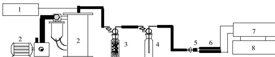
Figure 2. Schematic diagram of experimental apparatus. 1. vacuumeter, 2. vacuum pump, 3. dryer, 4. bumper, 5. tubular type reactor chamber, 6. electrode, 7. radio-power supply, 8. matching power supply.
