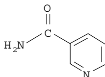
Scheme. The molecular structure of NA.
