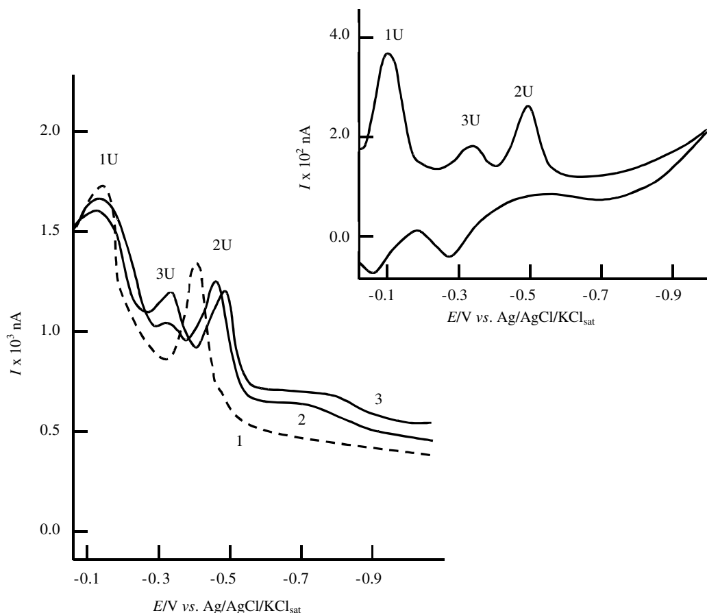
Figure 3. Square-wave voltammograms of 1 \times 10^{-5} \text{NH}_4\text{VO}_3 solution in the absence (---) and presence (—) of 5 \times 10^{-5} M (curve 2) and 1 \times 10^{-4} M (curve 3) NA in 0.1 M phosphate buffer (pH 7.4). 1U: the first reduction peak of free \text{NH}_4\text{VO}_3 ; 2U: the second reduction peak of free \text{NH}_4\text{VO}_3 ; 3U: the reduction peak of V(V)-NA complex. Experimental conditions as in Figure 1 (Upper: cyclic voltammogram of 1 \times 10^{-5} \text{NH}_4\text{VO}_3 solution in the presence 1 \times 10^{-4} M NA. Experimental conditions as in Figure 2).
