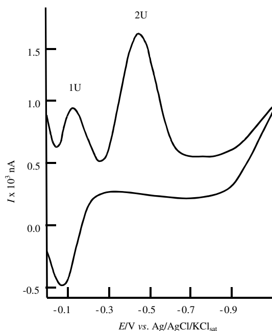
Figure 2. Cyclic voltammogram of 5 \times 10^{-5} M \text{NH}_4\text{VO}_3 solution in the phosphate buffer (pH 7.4). 1U: the reduction of V(V) to V(IV); 2U: the reduction of V(IV) to V(III). Experimental conditions: scan rate: 500 \text{ mV s}^{-1} ; scan increment: 2 mV; equilibrium time: 5 s; drop size: medium.
