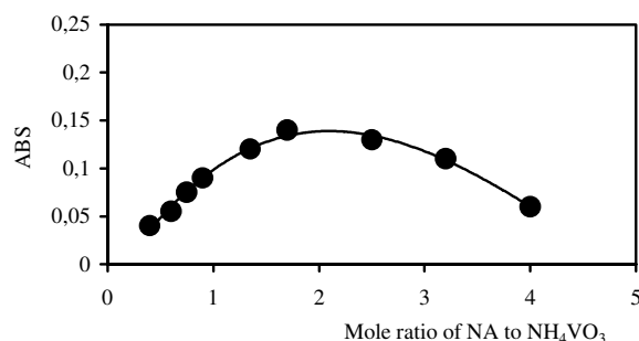
Figure 5. Plot of the absorbance at 415 nm versus the mole ratio of NA to NH 4 VO 3 .
