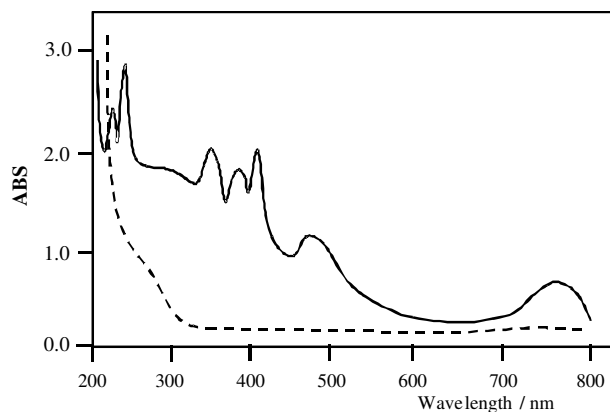
Figure 4. Absorbance spectra of 2 \times 10^{-4}\text{M} \text{NH}_4\text{VO}_3 solution (-----), and 1 \times 10^{-4}\text{M} \text{NH}_4\text{VO}_3 in the presence of 2 \times 10^{-4}\text{M} NA solution (—).
