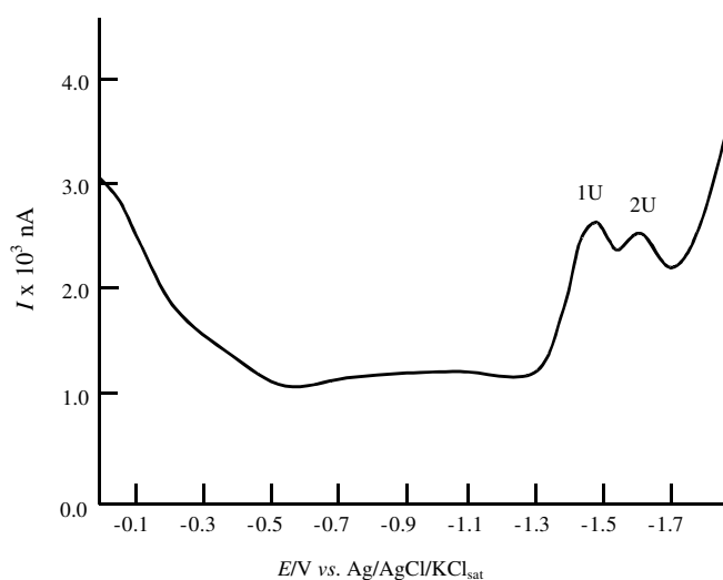
Figure 1. Square-wave voltammogram of 4.76 \times 10^{-4} M NA solution in the phosphate buffer (pH 7.4). 1U: the formation of the aldehyde derivative of NA ( -1.48 V); 2U: the formation of the carbinol derivative of NA ( -1.61 V). Experimental conditions: scan rate: 200 \text{ mV s}^{-1} ; equilibrium time: 5 s; frequency: 100 Hz; drop size: medium.
