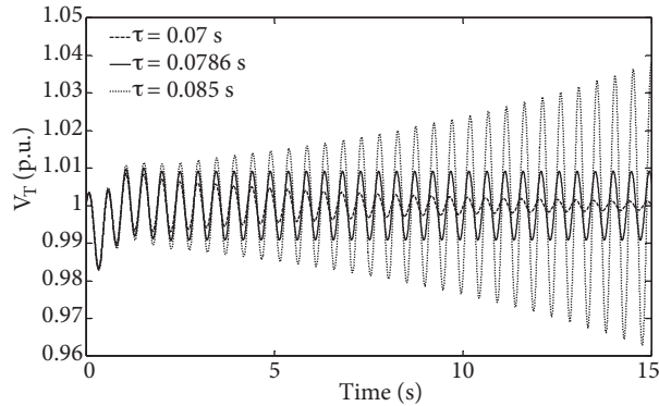
Figure 8. Generator terminal voltage for different time delays for K_P = 20 delay values around \tau_{1*} = 0.0786 \text{ s} for P_L = 0.5 \text{ pu} .
