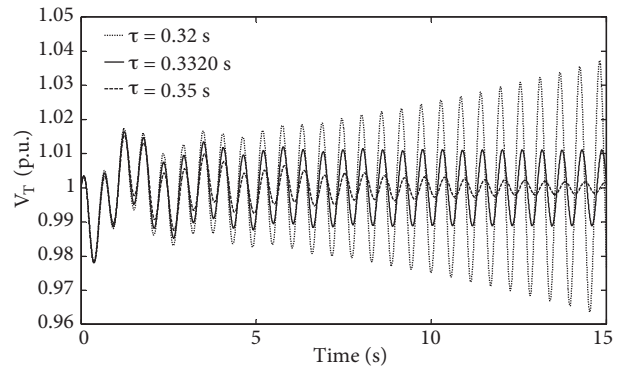
Figure 9. Generator terminal voltage for different time delays for K_P = 20 and delay values around \tau_{2*} = 0.3320 \text{ s} for P_L = 0.5 \text{ pu} .
