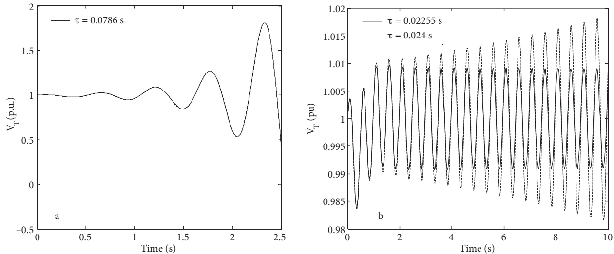
Figure 11. Generator terminal voltage for K_P = 20 , D = 0 , and P_L = 0.5pu when a delay is added into PSS loop.
