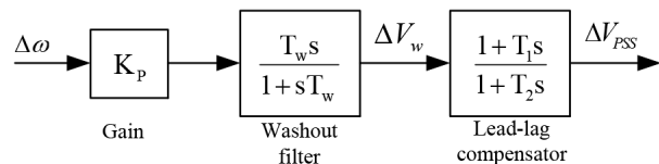
Figure 4. Block diagram of PSS [7,8,28].
