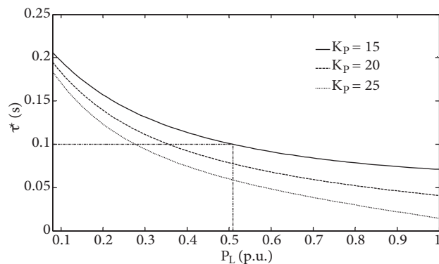
Figure 6. Variation of delay margin with respect to the load for different PSS gains.
