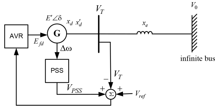
Figure 1. One-line diagram of SMIB with AVR and PSS [8,28].
