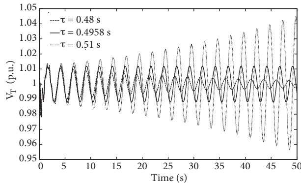
Figure 10. Generator terminal voltage for different time delays for K_P = 20 and delay values around \tau_{3*} = 0.4958 \text{ s} when D = 0 and P_L = 0.5 \text{ pu} .
