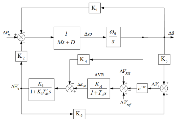
Figure 3. Detailed block diagram of the SMIB system with AVR including a time delay [8,28].
