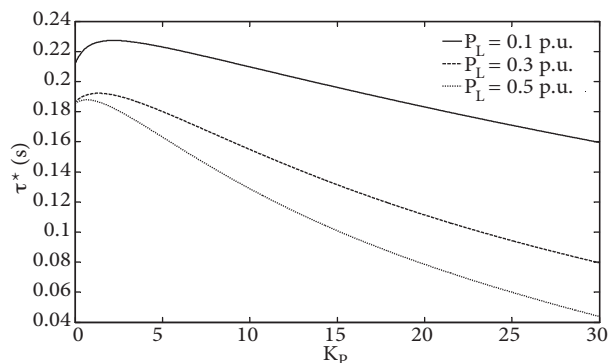
Figure 5. Variation of delay margin with respect to the PSS gain for different loads.
