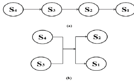
Figure 1. a) Conventional decoding, b) proposed decoding sequence of 2 × 2 MIMO system.
