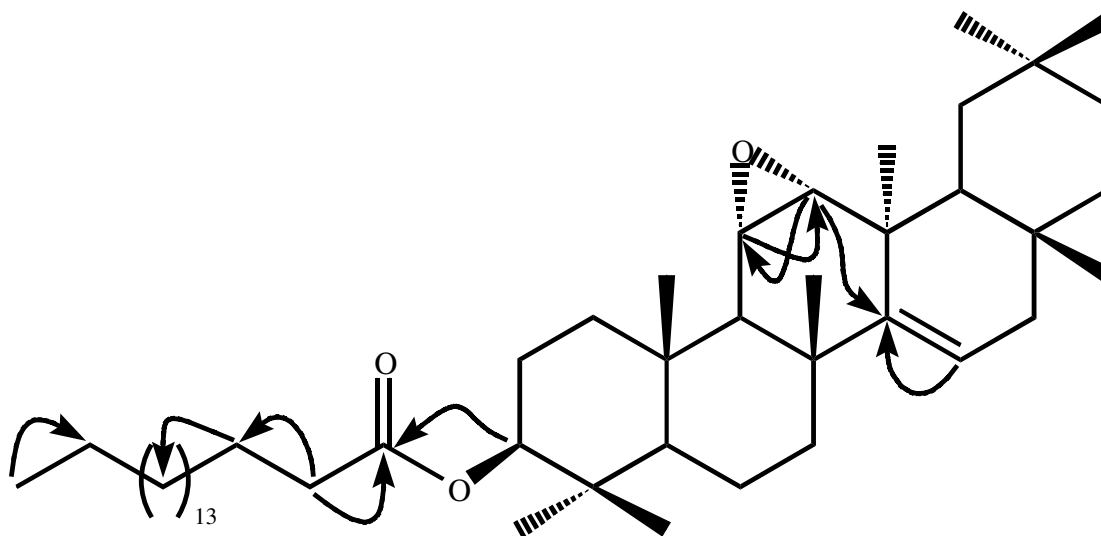
Figure 2. Important HMBC interactions in 2 .
