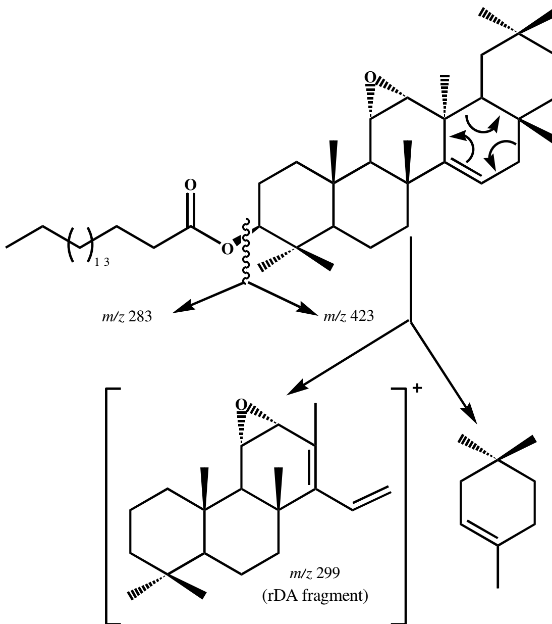
Scheme. Retro Diels-Alder (rDA) fragmentation in crassifoate ( 2 )
