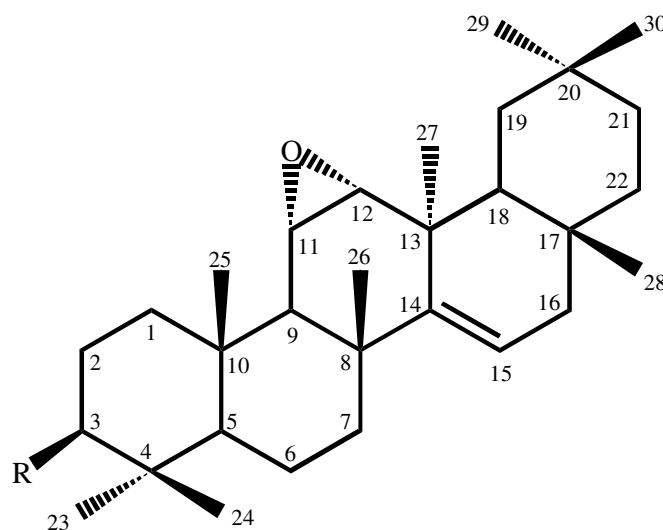
( 2 ) R = stearyl (crassifoate) ( 2a ) R = OH
