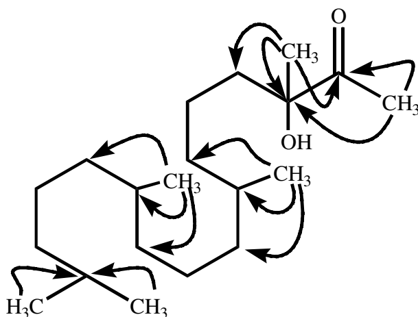
Figure 3. Important HMBC interactions in 3 .
