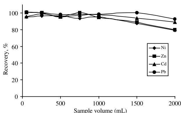
Figure 6. The effect of sample volume on the recovery of the metal ions (N = 3, RSD < 5%).
