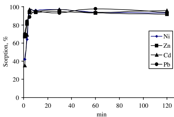
Figure 5. The rate of Pb 2+ , Cd 2+ , Ni 2+ , and Zn 2+ sorption on XAD-4-1,2-bis (o-aminophenylthio) ethane (N = 3, V = 50 mL, RSD < 5%).
