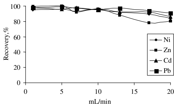
Figure 4. The effect of the flow rate of the solution ( N = 3 , V = 50 mL, RSD < 5\% ).
