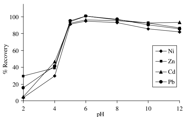
Figure 3. The effect of pH on the recovery of the metal ions ( N = 3 , V = 50 \text{ mL} , \text{RSD} < 5\% ).
