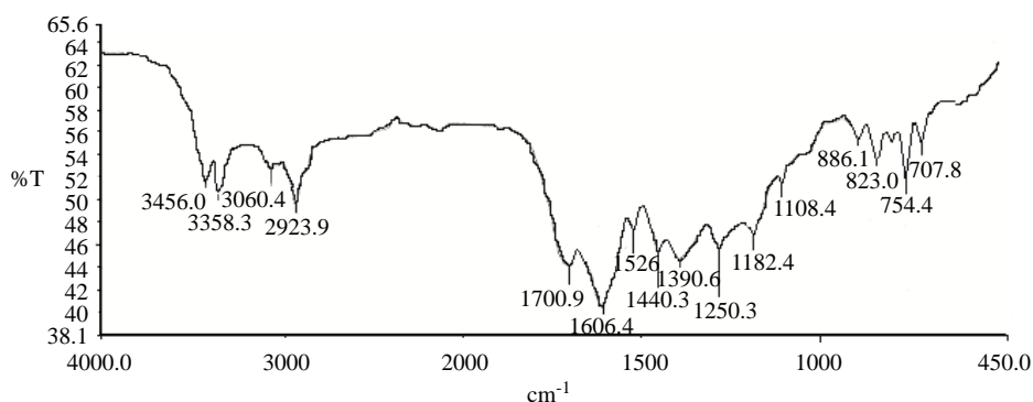
Figure 2. IR spectra of Amberlite XAD-4 resin functionalised with 1,2-bis (o-aminophenylthio) ethane.
