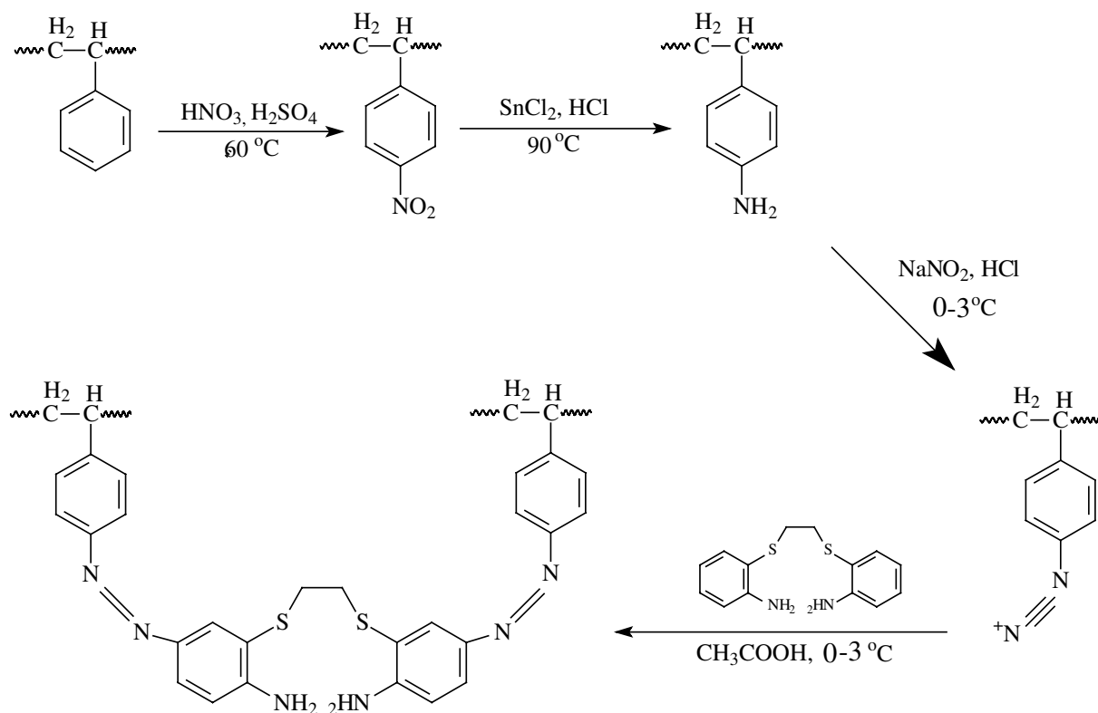
Figure 1. The synthesis and chemical structure of XAD-4-1,2-bis (o-aminophenylthio) ethane chelate resin.
